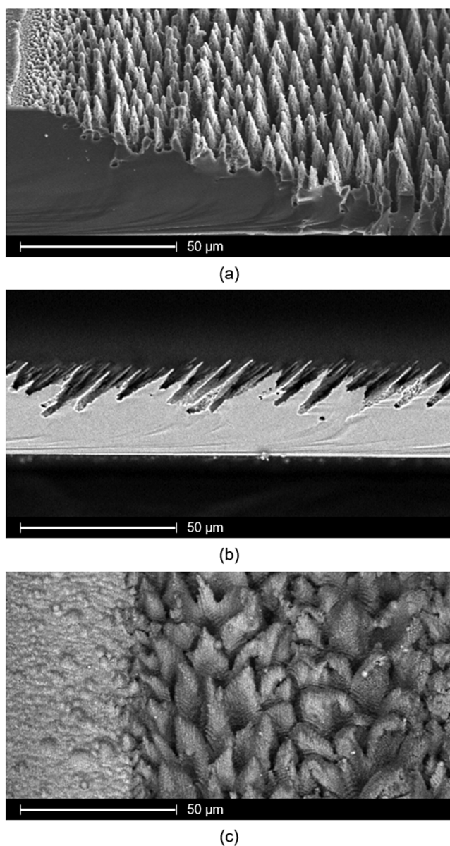
Figure 1. SEM images of laser-induced microstructures. The top and middle images show cross sections of Si processed in 600 mbar \text{SF}_6 . For (a) the pulse number was increased from 0 to 1500 pulses from left to right at a fluence of approximately 8 \text{ kJ m}^{-2} . The sample is viewed at 30^\circ . The slanted structures in (b) are created with a laser incidence angle of 45^\circ , a fluence of approximately 9 \text{ kJ m}^{-2} and roughly 1000 pulses. This sample is viewed at 90^\circ . The bottom image (c) shows Ti microstructures fabricated in 7 mbar vacuum with different laser fluences. Low fluences below the ablation threshold lead to ripples (left third) whereas higher fluences (up to 20 \text{ kJ m}^{-2} ) generate broad cones (two thirds on the right).
