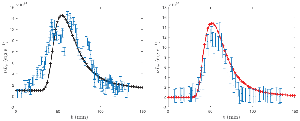
Figure 3. NIR and X-ray flare light curves of Sgr A*. Left panel: the black solid line is the theoretical NIR light curve. For comparison, the blue points with error bars present the observational data on 2007 April 4 (Dodds-Eden et al. 2009). Right panel: theoretical X-ray light curve (red) and the observed one (blue) during the same period.
