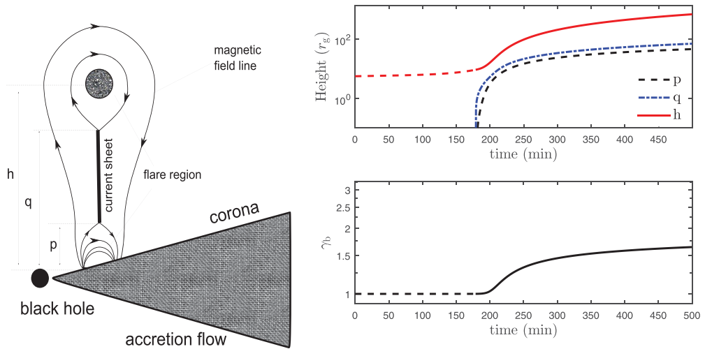
Figure 2. Left panel: Diagram of the flux rope configuration, showing the mathematical notation used in the text. The x -axis is parallel to the equatorial plane of the accretion flow, and the y -axis points upward. The bottom, top tip of the current sheet, and the height of the center of the flux rope are denoted by p , q , and h , respectively. All these heights are measured from the disk surface in our calculations. The distance between the magnetic source regions on the accretion flow is 2\lambda . Right panel (Upper): the red solid, blue, and black lines present the evolutions of the height of the flux rope h , and the current sheet ( q , p ) as a function of time. The red dashed line corresponds to the evolution prior to the loss of the equilibrium. Right panel (Bottom): the evolution of the Lorentz factor \gamma_b of the flux rope.
