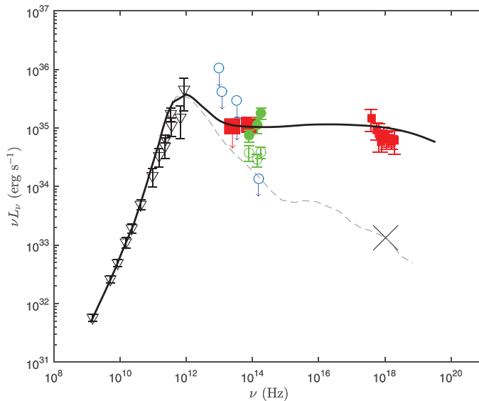
Figure 4. SED of Sgr A*. The observed data are quoted from Dodds-Eden et al. (2009). The filled red and green symbols present the flare state emission in infrared and X-ray, other data points correspond to the quiescent emission. The gray dashed line shows the RIAF model for the quiescent state emission from Yuan et al. (2003). The thick solid black line is the total model SED from synchrotron emission for Sgr A* after taking account of the quiescent emission.
