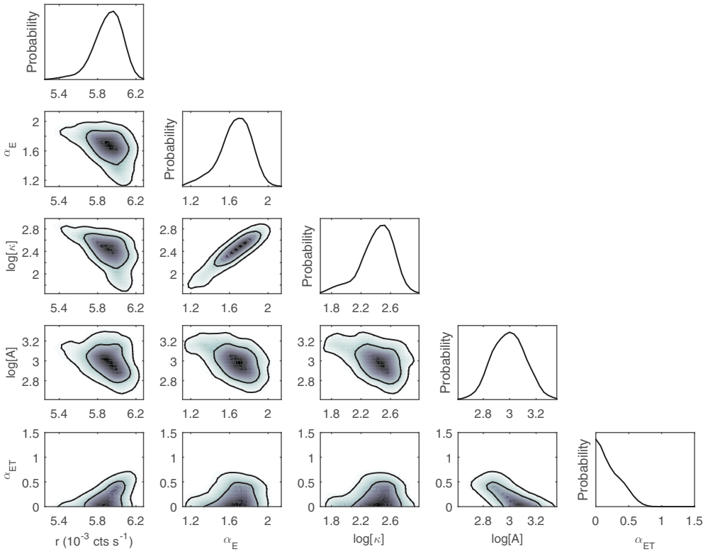
Figure 1. 1D and 2D probability distributions of the fitting parameters. The contours in the 2D plots are for confidence levels 68% and 95% from inside to outside, respectively.
