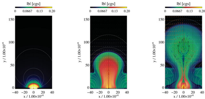
Figure 2. Snapshots of the MHD simulation of a solar flare showing the magnetic field strength (colours), field lines (white), and velocity vectors at (left to right) t = 0 , t = 3000 s, t = 4000 s.
