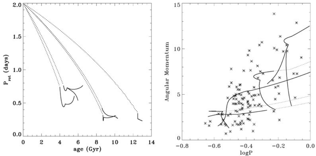
Figure 1. Computed time variations of orbital period of binaries with masses (from left to right): 1.3+1.1 , 1.3+1.0 , 1.0+0.8 , 1.0+0.5 and 0.9+0.45 M_{\odot} (left) and AM variations of the same binaries compared to the observed values of over 100 W Uma-type stars. Dotted lines denote detached stage and solid lines the contact phase.
