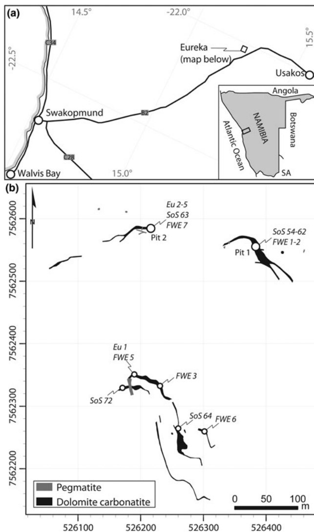
Fig. 1. Location map (a) and geological sketch map (b) of the Eureka carbonatite dykes, with pit and sample locations. Host rocks are quartzite and schists of the Etusis formation. Geological map grid is UTM 33S, WGS 1984 datum, redrawn and georeferenced from Dunai (1989).
