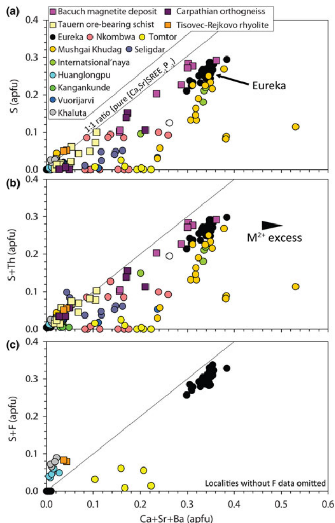
Fig. 7. Composition of monazite-(Ce) from Eureka compared with data compiled from other carbonatite complexes (circles; Kukharensko et al. , 1961; Cressey et al. , 1999; Bulakh et al. , 2000; Doroshkevich et al. , 2001; Wall, 2004; Lazareva et al. , 2015; Enkhbayar et al. , 2016; Prokopyev et al. , 2017; Nikolenko et al. , 2018), the Internatsional'naya kimberlite (Chakhmouradian and Mitchell, 1999), and other published occurrences (squares) with \text{SO}_3 > 1\% (Ondrejka et al. , 2007; Pršek et al. , 2010; Krenn et al. , 2011; Ondrejka et al. , 2016).
