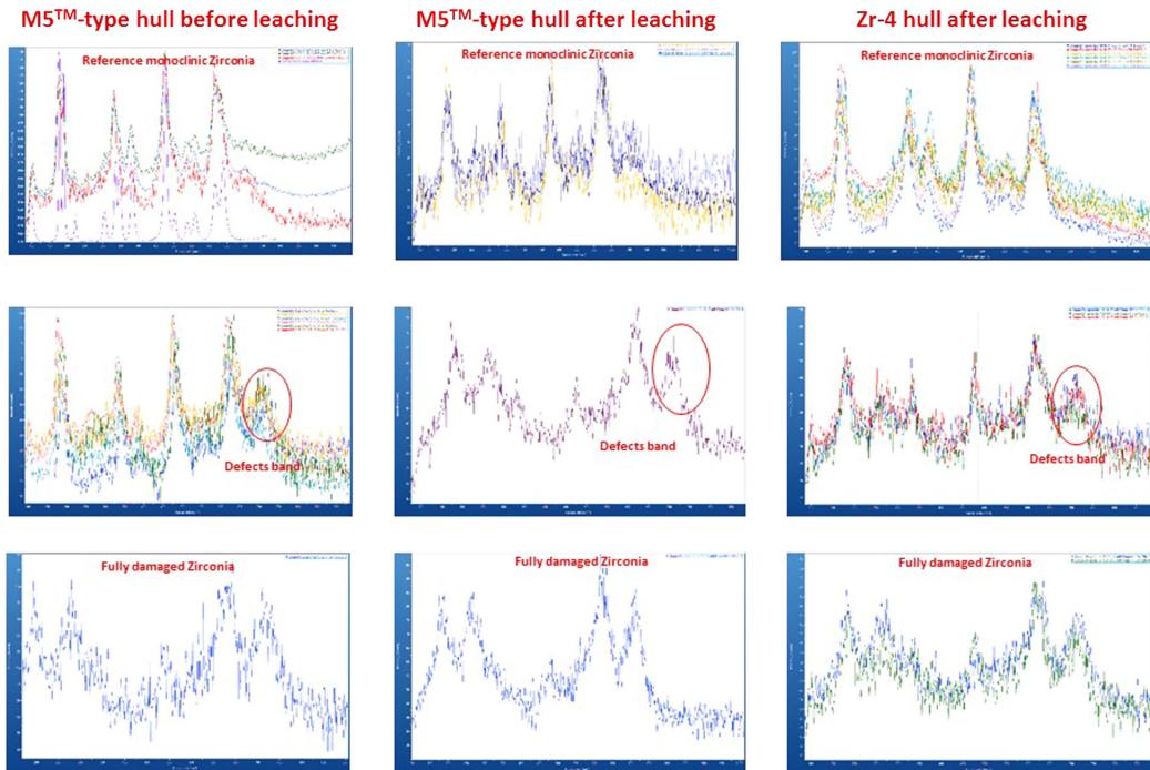
Figure 11 Raman spectra obtained on M5™ and Zr-4 hulls before and after leaching for 6 months in deaerated NaOH solution.
