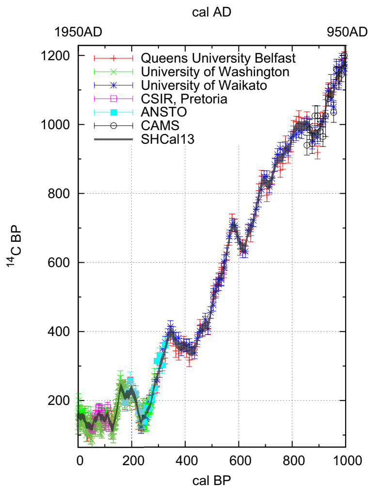
Figure 1A SHCal13 terrestrial calibration curve (1-standard deviation envelope) and data with 1-standard deviation uncertainty in the ^{14}\text{C} and calendar ages. Color-coded individual data sets can be seen in the online version of this article.
