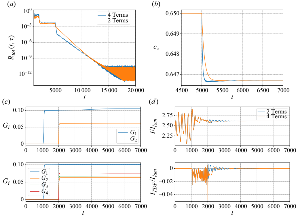
Figure 9. Successful stabilisation of UB at Re = 3000 from a turbulent state using MTDF (4.3) with two terms ( \tau_1 = 2, \tau_2 = 9 ) and four terms ( \tau_1 = 2, \tau_2 = 9, \tau_3 = 17, \tau_4 = 33 ). Panels show (a) R_{tot} , (b) c_z , (c, top) G_i with two terms, (c, bottom) G_i with four terms, (d) I/I_{lam} and I_{TDF}/I_{lam} . The gain, G_1(t) , is switched on at t = 1000 . Here, G_1(t) is initially increased following the sigmoid gain function (3.2) where (t_s, G_1^{max}, a, b) = (1000, 0.1, 0.1, 100) . At t = 2000 , the G_i parameters begin to evolve using the adaptive gain method as described by (5.6), with a constant value of \gamma_i^G = 0.1 applied to all delay terms. The adaptive shift method is switched on at t = 5000 , where \gamma^s = 0.1 and c_z(0) = 0.65 .
