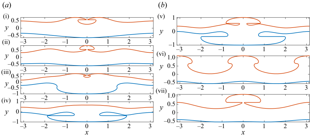
Figure 12. Almost limiting wave profiles corresponding to the labelled solutions (i) to (vii) in figure 11.
