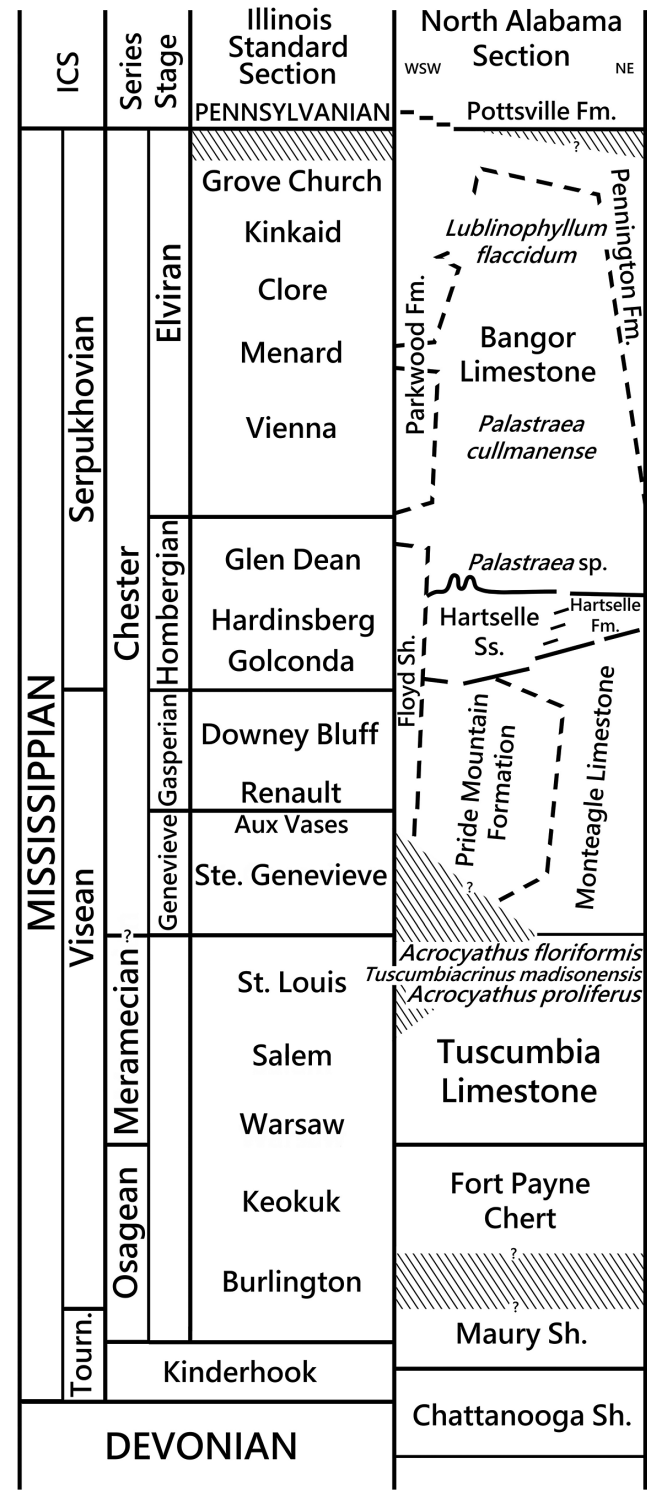
Figure 5. Mississippian stratigraphic section in northern Alabama compared to the Illinois Standard section. Position of Tuscumbiacrinus madisonensis n. gen. n. sp. is indicated as are key biostratigraphically important colonial coral intervals, including Acrocyathus proliferus (Hall in Hall and Whitney, 1858); Acrocyathus floriformis d'Orbigny, 1850; Palatraea cullmanense Rodríguez and Kopaska-Merkel, 2014; and Lublinophyllum flaccidum (Easton, 1943) (coral).
