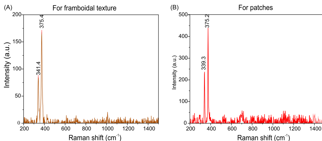
Figure 5. The Raman spectrum of the coatings observed on foraminiferal tests displays prominent peaks at \sim 375 and 340\text{ cm}^{-1} , indicating the presence of the pyrite phase (after Lara et al. 2015). The spectrum is illustrated in two forms: (A) Raman spectra for framboidal pyrite and (B) Raman spectra for the patchy pyrite.
