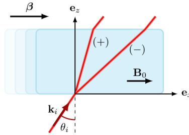
FIGURE 8. The incident wave is in the plane formed by the background magnetic field \mathbf{B}'_0 = \mathbf{B}_0 permeating the magnetised plasma and the direction of motion \beta . The rest-frame modes are the two solutions (+) and (-) for oblique propagation.
