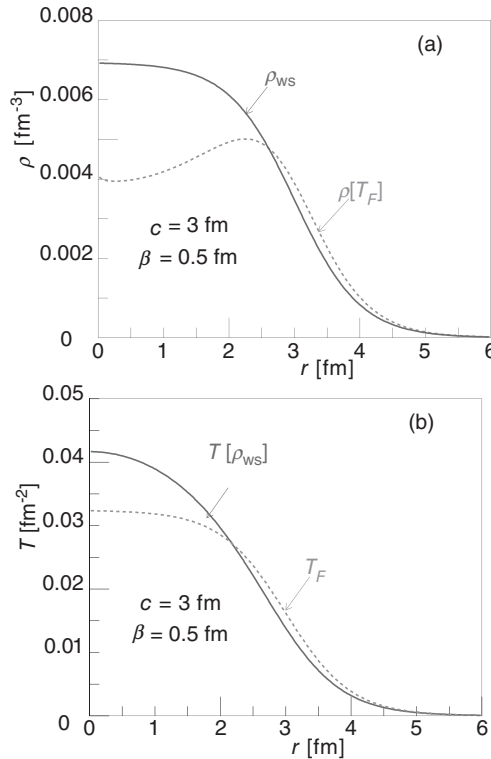
Figure 8.14 (a) A comparison of the Woods–Saxon density, \rho_{WS}(r) = \rho_0/[1 + \exp[(r-c)/\beta]] , with the density corresponding to the “Fermi” phase shift function (or a “Fermi” thickness function), \rho[T_F] . The normalization is \int d^3r \rho(r) = 1 . The shape parameters, c and \beta , are the same in both cases. (b) A comparison of the thickness function corresponding to the Woods–Saxon density, T[\rho_{WS}] , with the “Fermi” thickness function, T_F = T_0/[1 + \exp[(b-c)/\beta]] . The normalization is \int d^2b T(b) = 1 . Again the shape parameters are the same.
