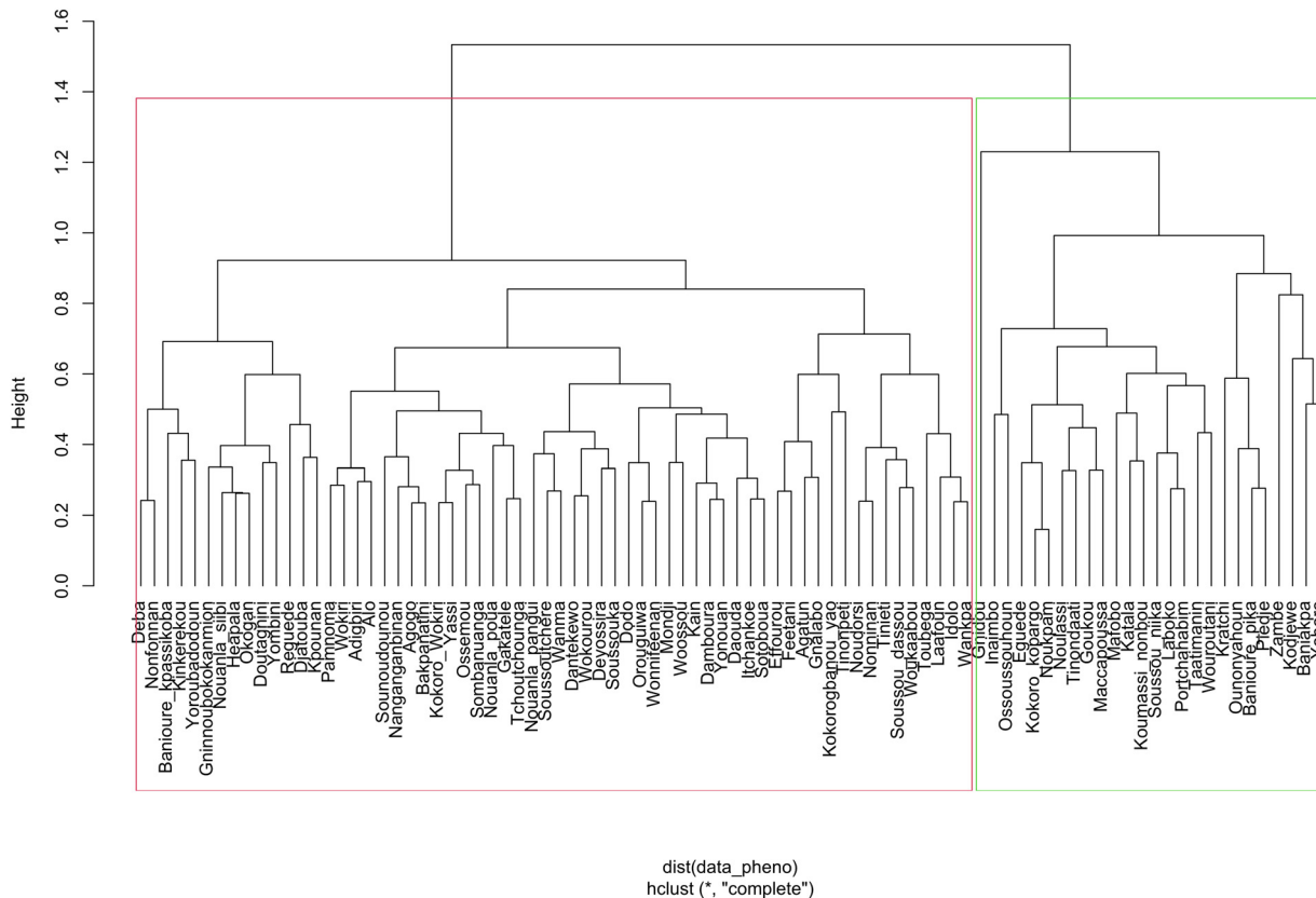
Fig. 1. Phenotypic characterization of Beninese white Guinea yam varieties based on Gower dissimilarity matrix using the 30 most discriminating traits. The colours represent the two clusters: Cluster 1 (red) and cluster 2 (green).
