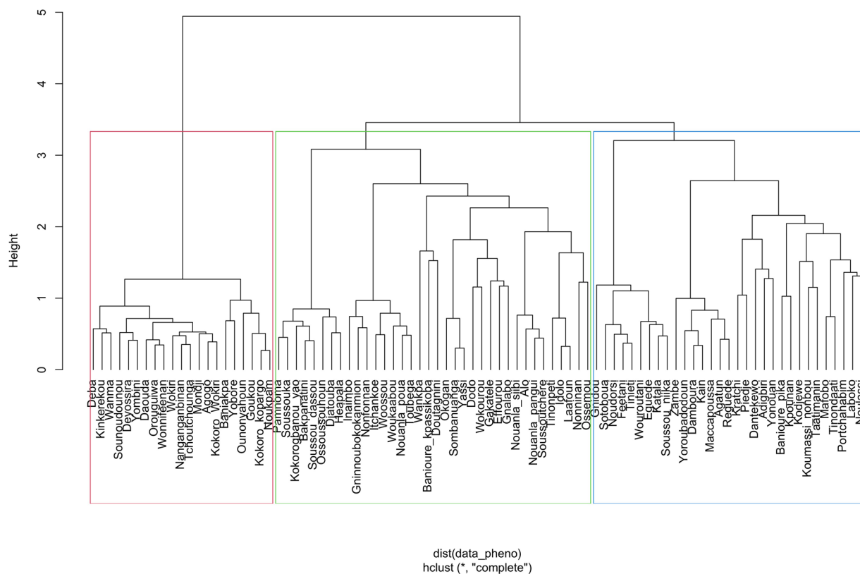
Fig. 4. Assessment of the genetic diversity among Beninese white Guinea yam accessions through the joint dissimilarity matrix. The colours represent the three clusters: Cluster 1 (red), cluster 2 (green) and cluster 3 (blue).
