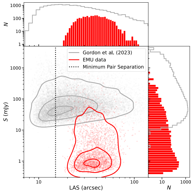
Figure 4. Distributions of LAS and integrated flux density ( S ) for likely DRAGNs in the EMU G09 field. Density contours of the distributions of LAS and S for EMU DRAGNs (red) for the VLASS DRAGNs (grey). Contours contain 90%, 50%, and 10% of the data points. The black dotted line represents the minimum pair separation ( 15'' ) used to select DRAGNs in this work. The difference between these distributions likely arises from the observational differences between EMU and VLASS.
