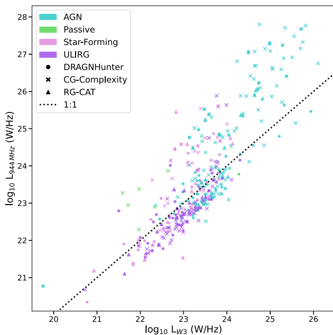
Figure 21. Radio luminosity versus W3 luminosity for sources identified by each source-finder, colour-coded by WISE-colour classification (passive, star-forming, ULIRG, AGN). The dashed line shows the 1:1 reference, included as a visual guide only and not representing the true radio-IR correlation (better traced by the distribution of star-forming sources). Most sources lie above the line, indicating a radio excess consistent with AGN-dominated emission, even for hosts classified as star-forming. Only sources with S/N > 3 in W1 , W2 , and W3 are shown.
