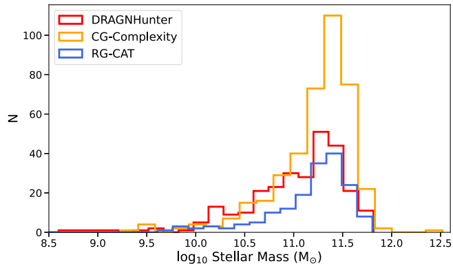
Figure 19. Stellar mass distributions of DH , CG-Complexity and RG-CAT sources cross-matched with GAMA-DR4 data (red, orange, and blue solid lines, respectively). All three distributions are broadly similar, peaking around 10^{11.4} M_{\odot} .
