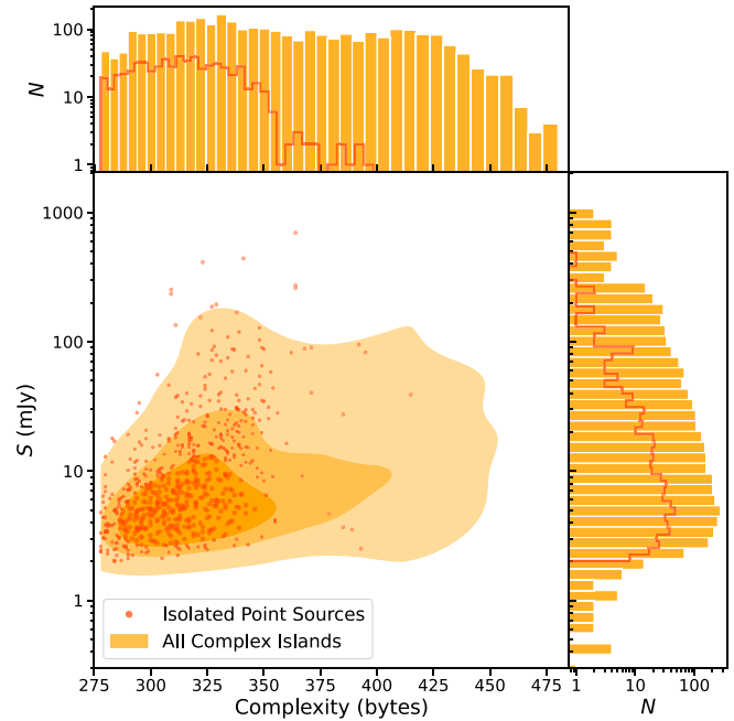
Figure C1. Distributions of complexity and flux density ( S ) for the entire high-complexity sample (orange) and isolated point sources within the high-complexity sample (dark orange). Density contours of the distributions of complexity and S for the full high-complexity sample contain 90%, 50%, and 25% of the data points.
