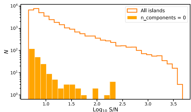
Figure B1. Signal to noise distributions of all islands (dark orange line) and islands with zero fitted components (orange bars).
