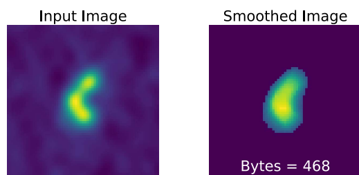
Figure 5. Illustrative example of the coarse-grained complexity process. An input image (left) is smoothed by a Gaussian filter to produce the smoothed image (right) which is then compressed using gzip. The byte length is then used as a proxy for apparent complexity of the radio source. The images here are 64 \times 64 pixels, corresponding to an angular size of 128'' \times 128'' .
