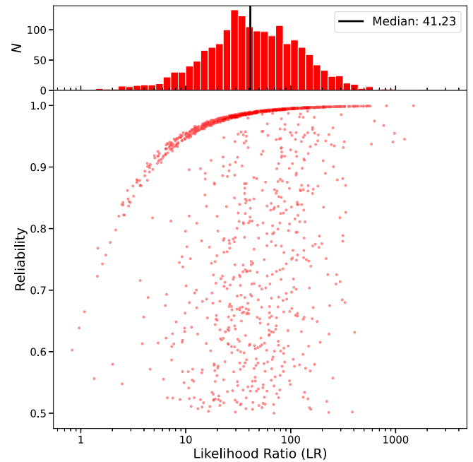
Figure D1. Top panel: Distribution of likelihood ratio values for DH sources cross-matched with AllWISE sources. Bottom panel: Likelihood ratio vs the calculated reliability for each cross-match.
