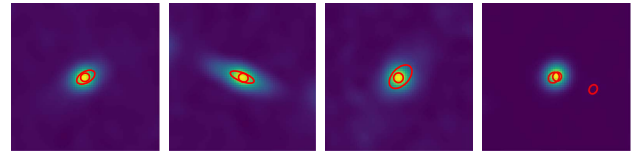
Figure A1. Sources with the lowest component pair separation. Overplotted are ellipses corresponding to the Gaussian components fit by Selavy . For each of these sources, the components are nested, therefore producing extremely small component pair separation. All cutouts are 64 \times 64 pixels, corresponding to an angular size of 128'' \times 128'' .
