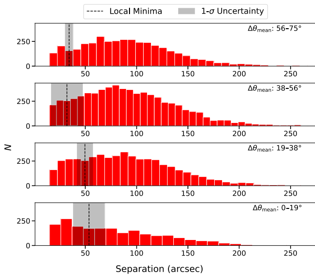
Figure 2. Distributions of angular separation of identified pairs in EMU-G09 (red bars) in bins of mean misalignment. Black lines mark the local minima, with the shaded region showing the 1\sigma uncertainty of their positions.
