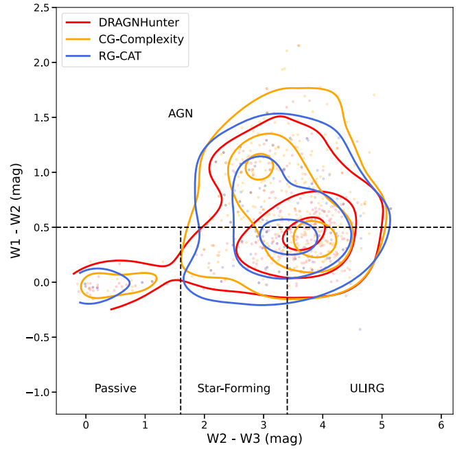
Figure 20. The WISE colour distributions for the hosts of sources identified by DH (red), CG-Complexity (orange), and RG-CAT (blue). The contours contain 90%, 50%, and 10% of the data points. Despite differences in detection strategy, sources identified by all three approaches have similar infrared host populations, with many sources classified in the star-forming/ULIRG region of WISE colour space. Note, only sources with a S/N > 3 in W1 , W2 , and W3 are shown.
