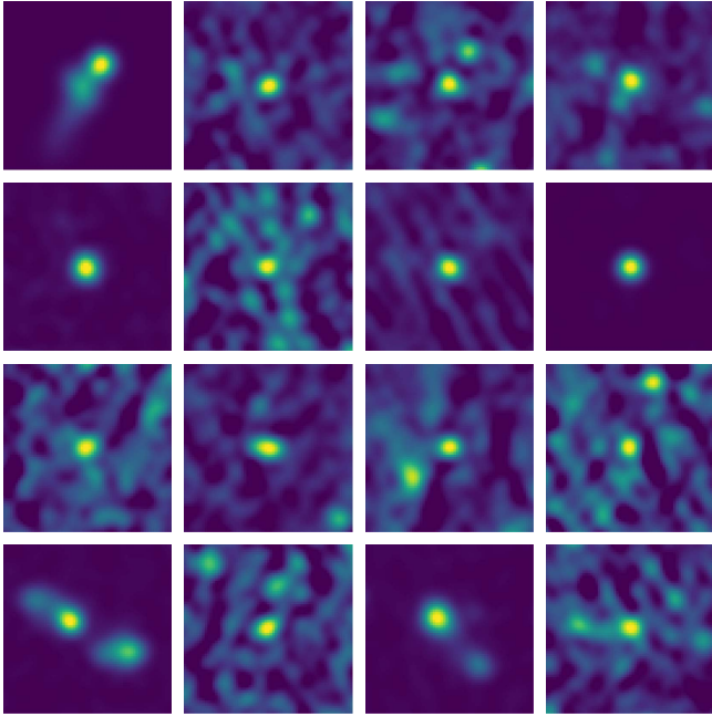
Figure B2. Cutouts of a random selection of 16 islands with zero fitted Gaussian components. All cutouts are 64 \times 64 pixels, corresponding to an angular size of 128'' \times 128'' .
