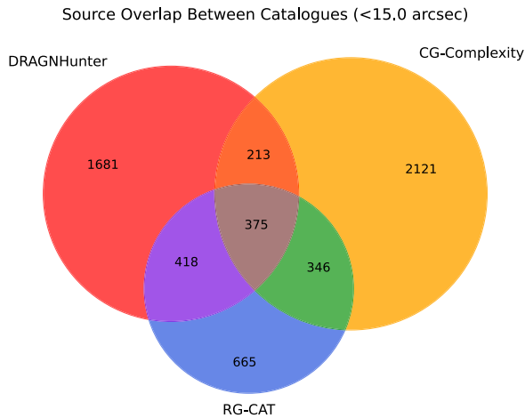
Figure 12. Overlap ( < 15'' ) of sources detected by DRAGNHUNTER (red), CG-Complexity (orange), and RG-CAT (blue). Each region of the diagram represents the number of sources uniquely or jointly identified by the corresponding source-finders. Only 375 sources are common to all three, with this small overlap likely reflecting the differing selection biases of each method.
