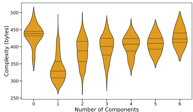
Figure 6. Source complexity as a function of the number of components fit to each Selavy island, with quartiles marked inside. Note the general trend of increasing complexity with the number of components.
