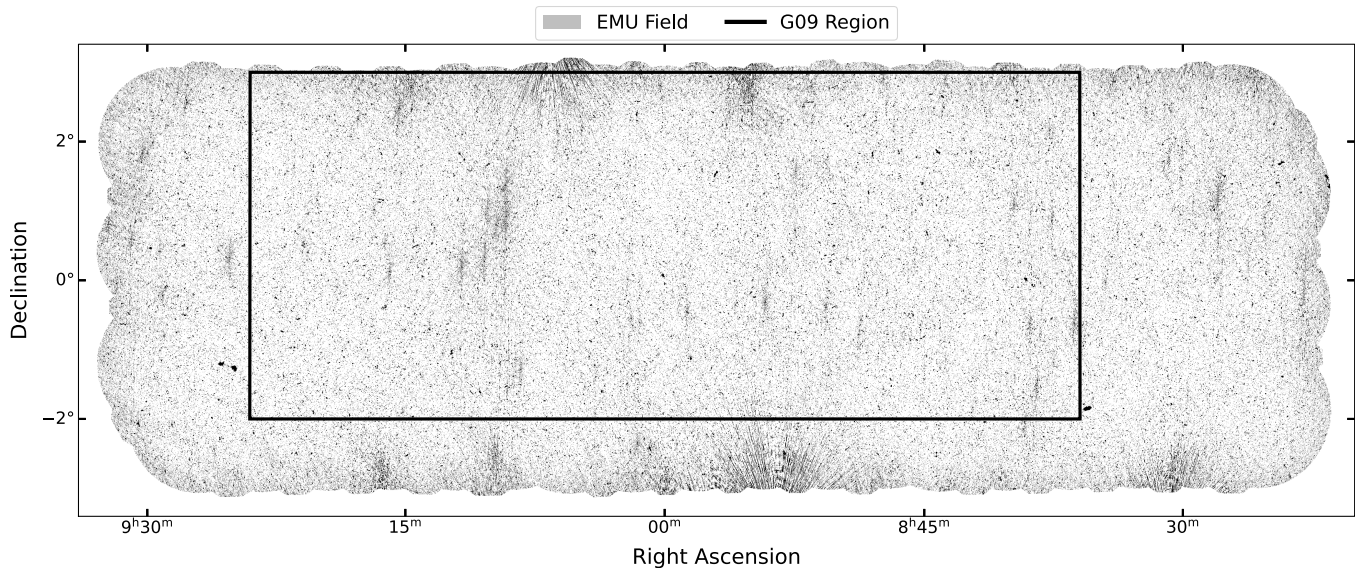
Figure 1. EMU mosaic constructed from the three EMU tiles that overlap the GAMA09 region with the black box indicating the GAMA09 footprint. The EMU observations are centred on a frequency of 944 MHz, a native resolution of 11'' \times 13'' , and an rms sensitivity of \sim 25 \mu\text{Jy beam}^{-1} . These data constitute the EMU-G09 region used throughout this paper.
