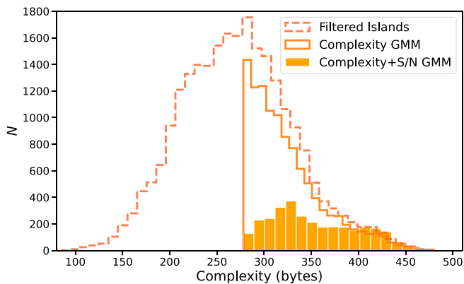
Figure 7. Comparison of distributions of the coarse-grained complexity values for all islands (dark orange dashed line), the complexity-only GMM (orange line), and the complexity+S/N GMM (light orange solid bars).
