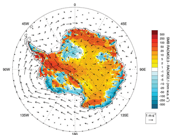
Fig. 4. Average (1979–2011) SMB difference (RACMO2.3 – RACMO2.1). Vectors show direction and magnitude of average 500 hPa wind speed difference (RACMO2.3 – RACMO2.1) ( \text{m s}^{-1} ). Areas where the difference exceeds one unit of standard deviation of the difference are stippled.
