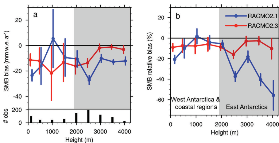
Fig. 5. (a) Absolute bias and (b) relative bias ((model–observation)/(model × 100%)) in modelled SMB for RACMO2.1 (blue) and RACMO2.3 (red). The data are binned in 500 m surface elevation intervals (0–250, 250–750 m, etc.). Error bars denote the combined uncertainty of the model and observations in each height bin, based on Van de Berg and others (2006). Elevations above 2000 m (shaded grey) represent East Antarctica exclusively. The bar chart in (a) denotes the amount of weighted observations in each bin. To separate blue and red lines, x-axis locations of each bin are displaced by 75 m.
