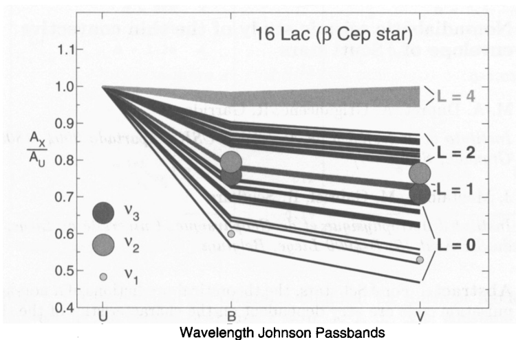
Figure 1. Theoretical (lines) and observational (circles) photometric amplitude ratios for three modes of 16 Lac. The theoretical amplitude ratios were computed for several models in the error box of the star in the HR diagram.
