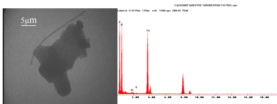
Figure 2.- Image and chemical composition of TSP obtained trough TEM
