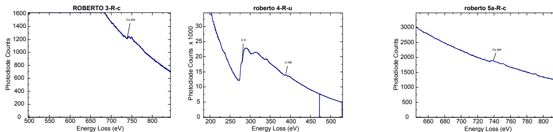
Figure 3.- EELS spectrum that shows the presence of C, U and Cs in particles
