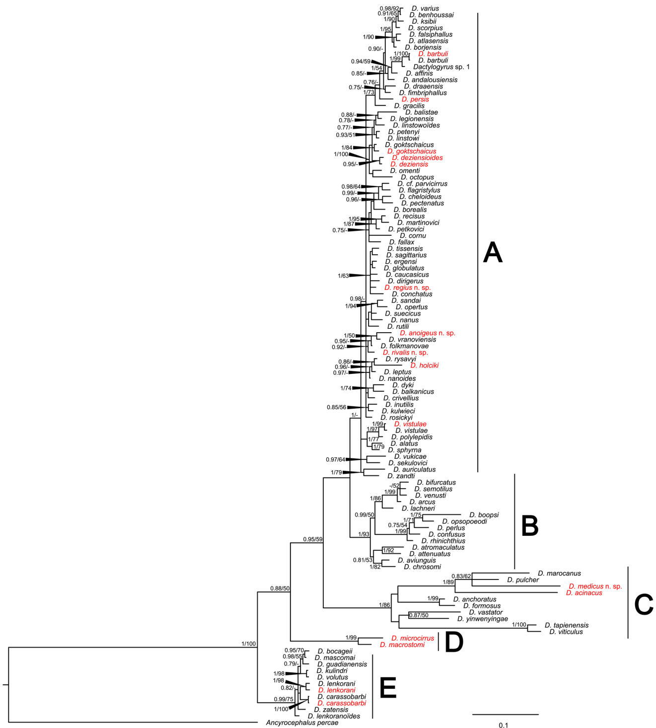
Figure 2. Phylogenetic tree of 105 Dactylogyrus spp. parasitizing various cyprinoid fish hosts. The tree is based on 111 combined sequences of partial genes coding 18S and 28S rRNA, and rooted using Ancyrocephalus percae . Values at the nodes indicate posterior probabilities from BI and bootstrap values from ML analyses. Dashes indicate values below 0.70 and 50, respectively. Letters (A–E) represent specific well-supported clades. The newly described and newly reported species from this study are in red.
