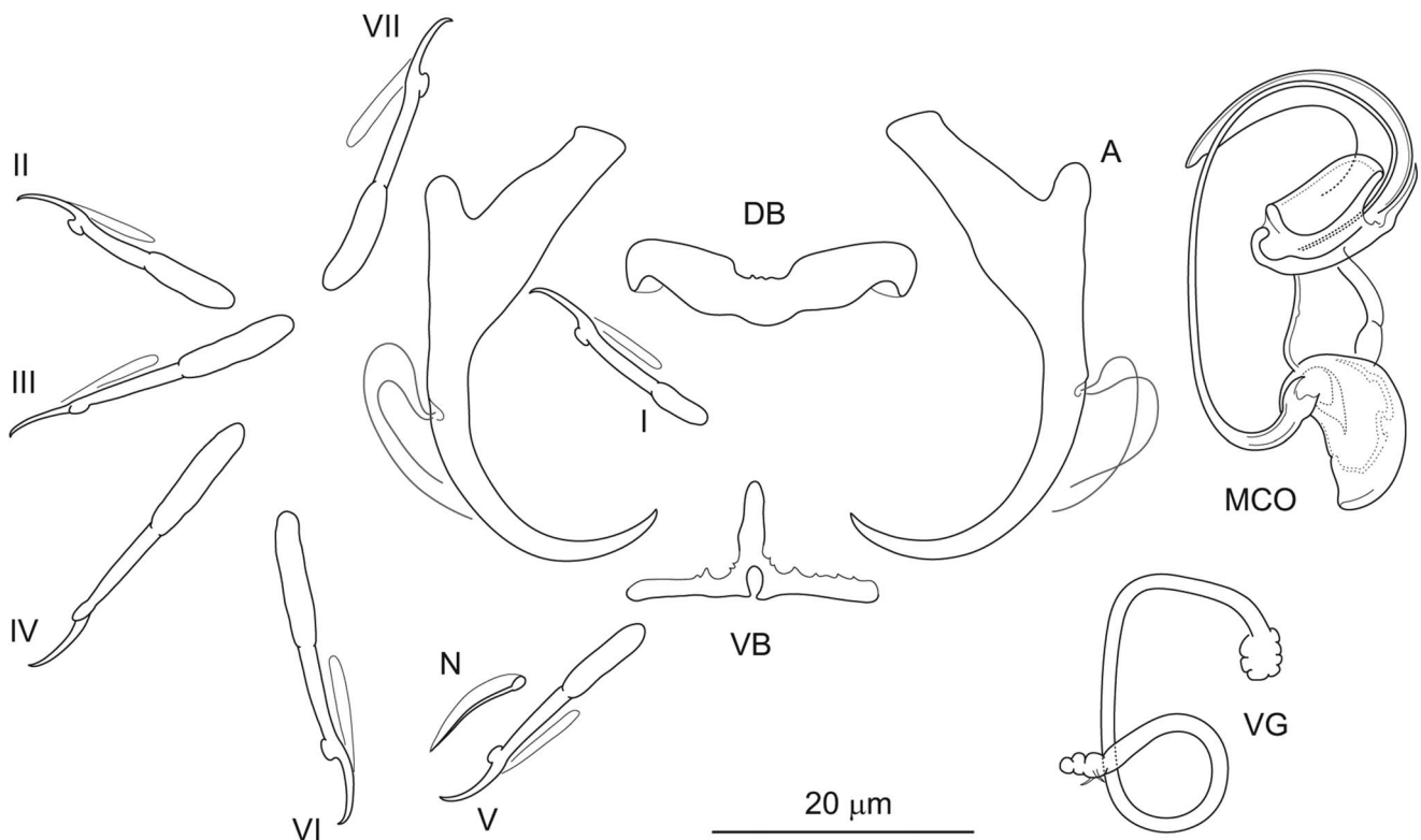
Figure 5. Hard structures of Dactylogyrus regius n. sp. ex Chondrostoma regium . A, anchor; DB, dorsal bar; VB, ventral bar; N, needle; I–VII, hooks; VG, vagina; MCO, male copulatory organ.
