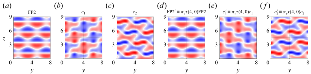
Figure 10. Equilibria and eigenmodes at Ra = 6218.6 . Case (a) FP2, (b) its unstable eigenmode e_1 and (c) its stable eigenmode e_2 . Case (d) \text{FP2}' = \pi_y \tau(4, 0)\text{FP2} , (e) its unstable eigenmode e_1' = \pi_y \tau(4, 0)e_1 and (f) its stable eigenmode e_2' = \pi_y \tau(4, 0)e_2 . The wavenumbers of the equilibria and eigenmodes in the y -direction suggest a 1 : 2 mode interaction.
