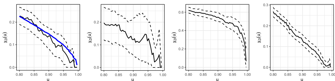
Figure 3. Examples of estimates of \chi_D(u) for four environmental datasets. Solid black lines represent point estimates, whereas dashed black lines are approximate 95% pointwise confidence intervals based on block bootstrapped estimates. From left to right: UKCP daily precipitation data from Figure 1 at d = 1024 sites (within the blue subregion shown in the left panel of Figure 1), with the model fit in blue (based on the Huser and Wadsworth, 2019 model fitted using a pretrained neural Bayes estimator); gridded conditionally simulated E-OBS Irish summer temperature data at d = 178 locations; (detrended) Red Sea surface temperature data at d = 144 locations in the Gulf of Aqaba; daily mean windspeed at d = 7 locations in the Vaucluse “département” in France.
