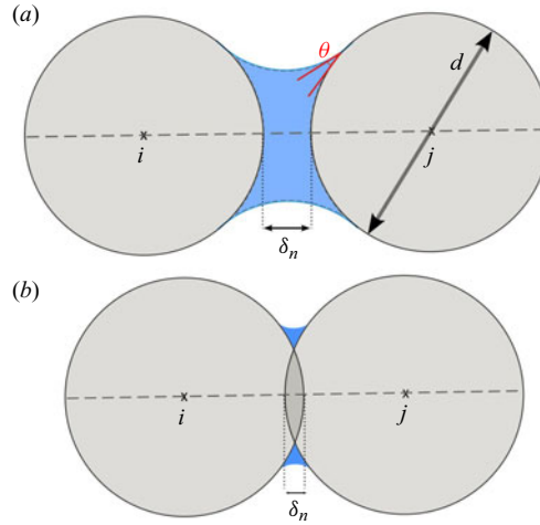
Figure 1. Geometry of a capillary bridge between two particles with gap (a) and overlap (b).
