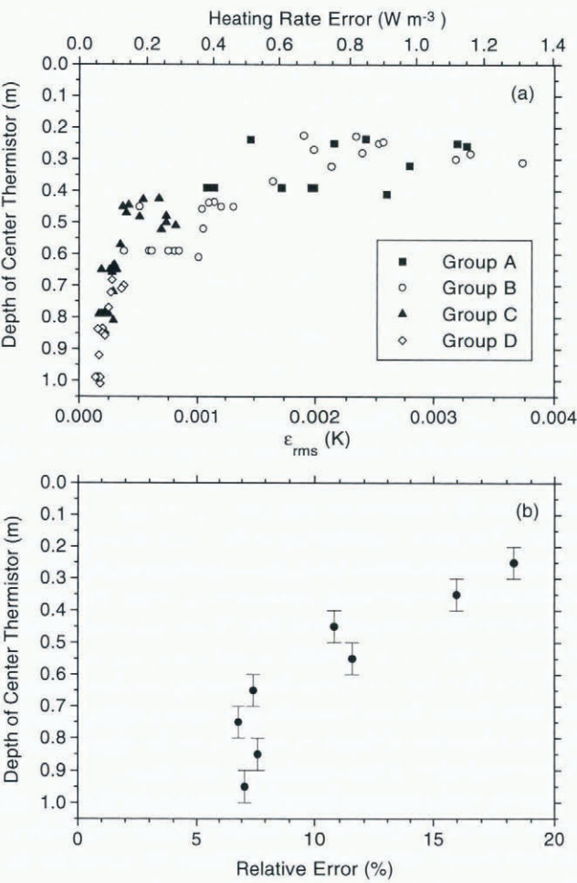
Fig. 12. (a) Root-mean-square error in predicted temperature change, \epsilon_{\text{rms}} (Equation (7)) as a function of depth for all thermistor groups for all periods of no sunlight. The top axis indicates the equivalent residual heating rate. The model uses the average conductivity for each group (horizontal lines in Figure 10). (b) Relative error in predicted temperature change, \epsilon_{\text{rms}}/\Delta T_{\text{rms}} (Equations (7) and (8)) vs depth, averaged over 10 cm intervals for all thermistor groups for all periods of no sunlight. The predicted temperature change was computed using the 6 month average conductivity for each group.
