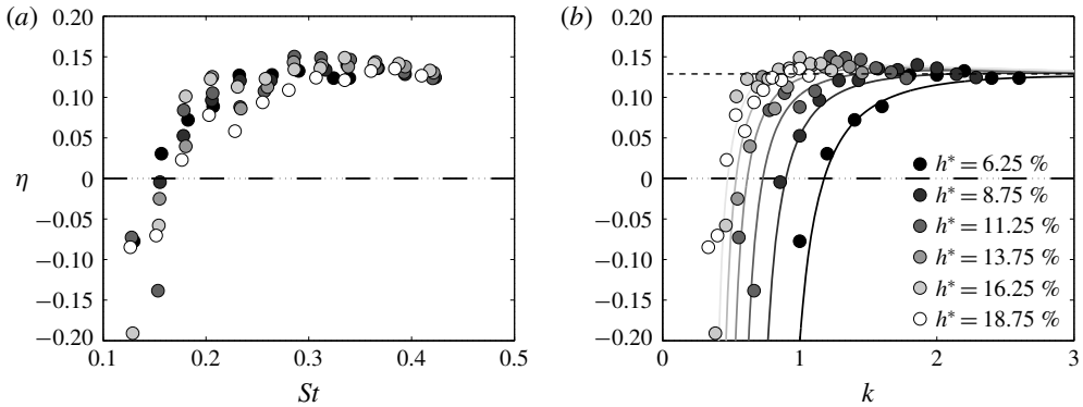
FIGURE 20. Heaving motions of a tear-drop shaped foil. Efficiency as a function of (a) Strouhal number St , and (b) reduced frequency k . In (b) solid lines indicate the scaling given by (3.10); short dashed line indicates the scaling with C_{Dh} = 0 and large k . Adapted with permission from Floryan et al. (2017a).
