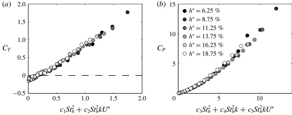
FIGURE 19. Heaving motions of a tear-drop shaped foil. Time-averaged (a) thrust and (b) power coefficients as functions of the scaling parameters (3.10) for various h^* = h_0/c . Adapted with permission from Floryan et al. (2017a).
