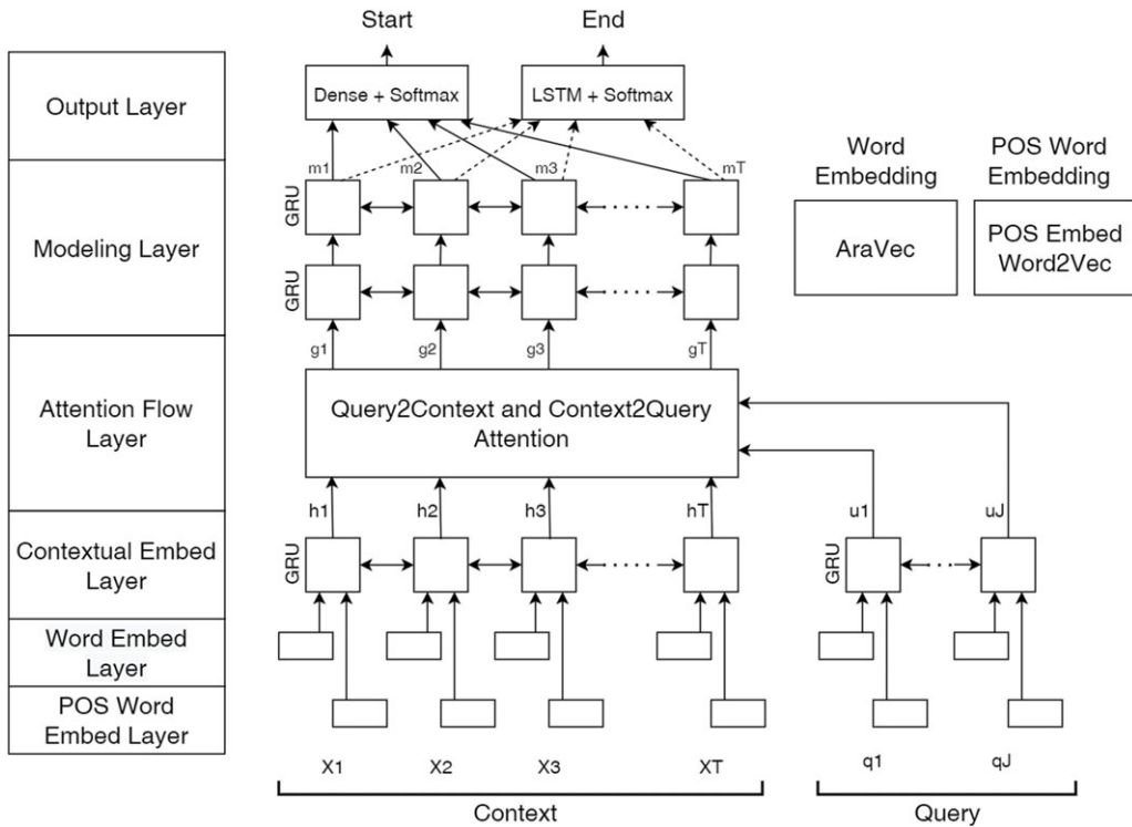
Figure 2. Improved-BIDAF Architecture.
