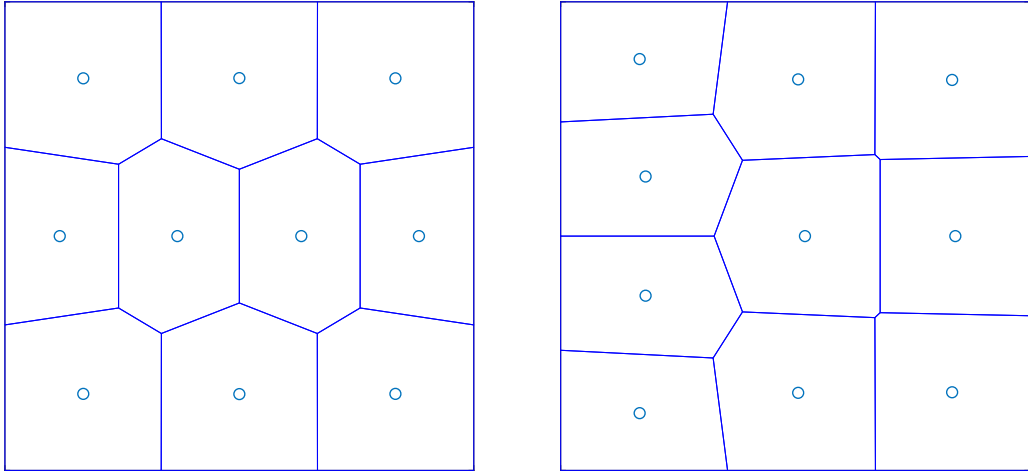
Figure 1. Two (approximate) centroidal Voronoi tessellations (CVTs) of 10 points for the uniform density \mu = 1 on a unit square. The polygons are the centroidal Voronoi cells V_i and the circles are the generators x_i . The CVTs were computed using Lloyd's algorithm. The CVT on the left has a lower energy J than the CVT on the right. The corresponding quantizer \nu = \sum_{i=1}^{10} m_i \delta_{x_i} of \mu is reconstructed from the CVT by taking m_i as the areas of the centroidal Voronoi cells and x_i as their generators.
