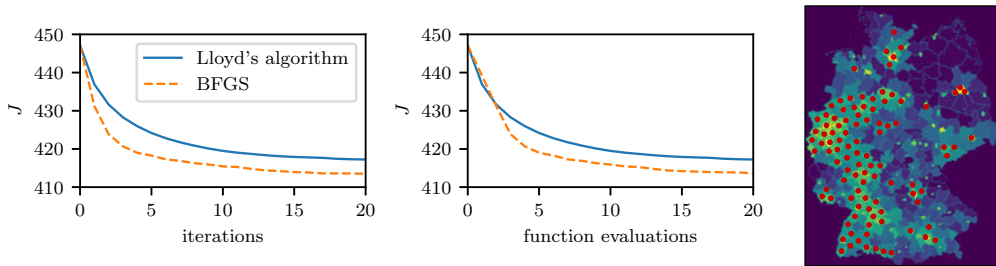
Figure 7. Quantization energy decrease of Lloyd's algorithm and a BFGS method versus number of iterations (left) and function evaluations (centre; for the BFGS method function evaluations differ from iterations due to additional evaluations in the stepsize control) for the example shown on the right. Right: Input density \mu and optimal locations (x_1, \dots, x_M) for M = 100 , where \mu is population density in Germany 2015 (published by the Federal Statistical Office of Germany in the "Regional Atlas" http://www.destatis.de/regionalatlas ). The computations use the Hellinger–Kantorovich model.
