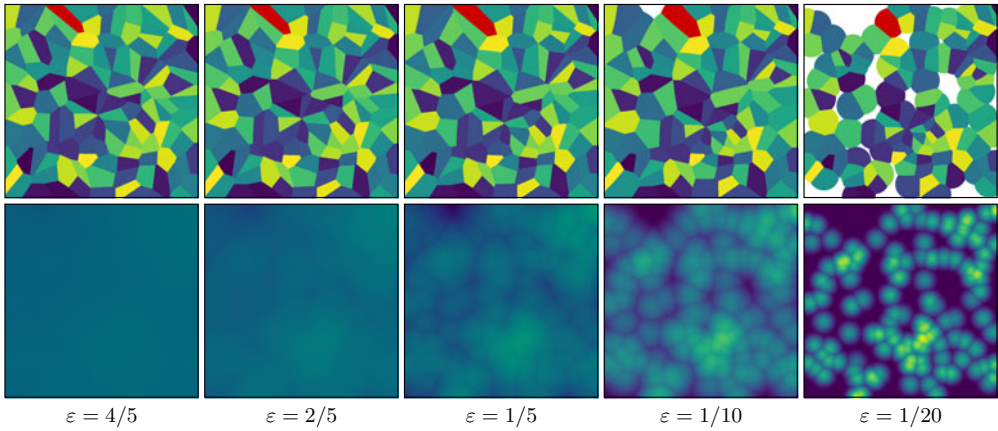
Figure 5. Semi-discrete Hellinger–Kantorovich distance on \Omega = [0, 1]^2 for different length scales \varepsilon , as in Figure 2, but for M = 128 . The evolution of one cell C_i(w) for fixed i is highlighted in red (top row). For large \varepsilon , C_i(w) is essentially the standard Wasserstein-2 Laguerre cell, not necessarily containing x_i . For small \varepsilon , C_i(w) becomes (a fraction of) the open ball B_{\varepsilon\pi/2}(x_i) .
