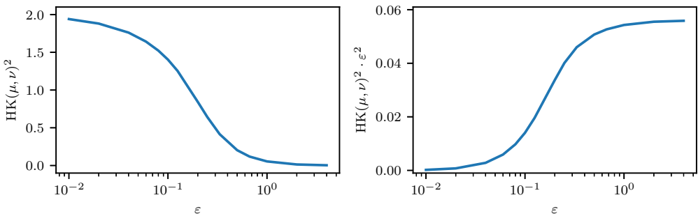
Figure 6. \text{HK}^\varepsilon(\mu, \nu)^2 for different length scales \varepsilon for the setup from Figure 2. Left: as \varepsilon \searrow 0 , \text{HK}^\varepsilon(\mu, \nu)^2 tends to \text{Hell}(\mu, \nu)^2 = 2 . Right: as \varepsilon \rightarrow \infty , \varepsilon^2 \text{HK}^\varepsilon(\mu, \nu)^2 tends to W_2(\mu, \nu)^2 .
