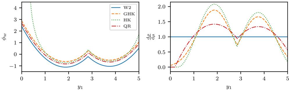
Figure 3. Semi-discrete transport between the Lebesgue measure on \Omega = [0, L]^2 , L = 5 and a discrete measure with M = 4 Dirac masses of locations (x_1, x_2, x_3, x_4) = L \cdot ((0.375, 0.375), (0.75, 0.35), (0.65, 0.75), (0.25, 0.8)) and weights (m_1, m_2, m_3, m_4) = |\Omega| \cdot (0.38, 0.29, 0.19, 0.14) . Top row: optimal cells \{C_i(w)\}_{i=1}^M ; the residual set R is represented by white; location of the discrete points (x_1, \dots, x_M) is indicated with red dots. Bottom row: optimal marginal \rho (identical colour scale in all figures; regions with \frac{d\rho}{d\mu}(x) = 0 are white for emphasis) and boundaries of cells \{C_i(w)\}_{i=1}^M (red) are shown for models (a)–(b) from Examples 2.9 and 3.14. Figure (e) shows the same model as (d), only with c(x, y) = [d(x, y)/2]^2 instead of c(x, y) = d(x, y)^2 ; on some cells \text{spt } \rho is now strictly bounded away from the boundaries of C_i(w) .
