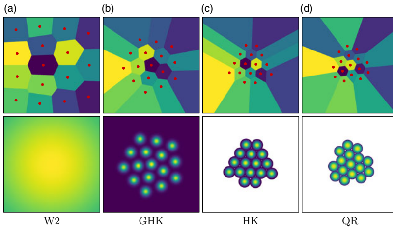
Figure 8. Quantization results for \mu = (1 + \exp(-\frac{|x|^2}{2(4\pi)^2})) \cdot \mathcal{L}_\Omega and \Omega = [-4\pi, 4\pi]^2 , M = 16 on the same models as in Figure 3. Top row: optimal locations x_1, \dots, x_M and Voronoi cells \{V_i(x_1, \dots, x_M)\}_{i=1}^M . Bottom row: optimal marginal \rho = \pi_{1\#}\gamma (identical colour scale in all figures; regions with \frac{d\rho}{d\mu}(x) = 0 are white for emphasis). For (a) we have \rho = \mu .
