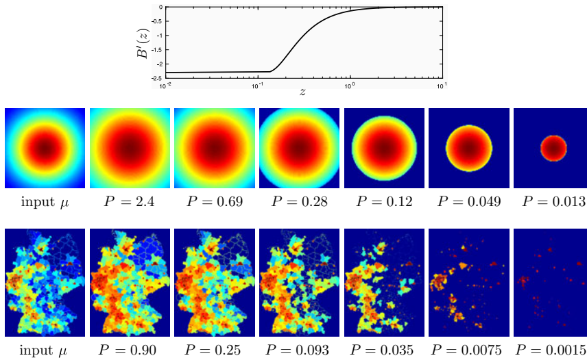
Figure 11. Top row: B' from Lemma 4.14 for Hellinger–Kantorovich transport. Middle and bottom row: input distribution \mu (a Gaussian and same data as in Figure 7) as well as asymptotically optimal point densities D for different values of P = \lim_{M \rightarrow \infty} \varepsilon_M^2 M (colour-coding from blue for 0 to red for maximum value).
