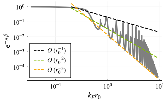
Figure 4. Dependence of the wave damping factor over half an orbital period, denoted e^{-\pi\beta} = e^{-T_O/(2T_M)} , at the onset of instability on the orbital radius, r_0 , for a linear central force, \mathbf{F} = -k\mathbf{x}_p ( n = 1 ). The grey curve is a rescaling of the stability boundary (white curve) presented in figure 3(d). Notably, the envelopes of the instability tongues satisfy the scaling e^{-\pi\beta} = O(\hat{r}_0^{-l}) for l = 2 and l = 3 , which are used in the asymptotic analysis presented in § 4.1. The scaling e^{-\pi\beta} = O(\hat{r}_0^{-1}) emerges between pairs of instability tongues, including for 3-wobbles, but is outside the scope of this investigation.
