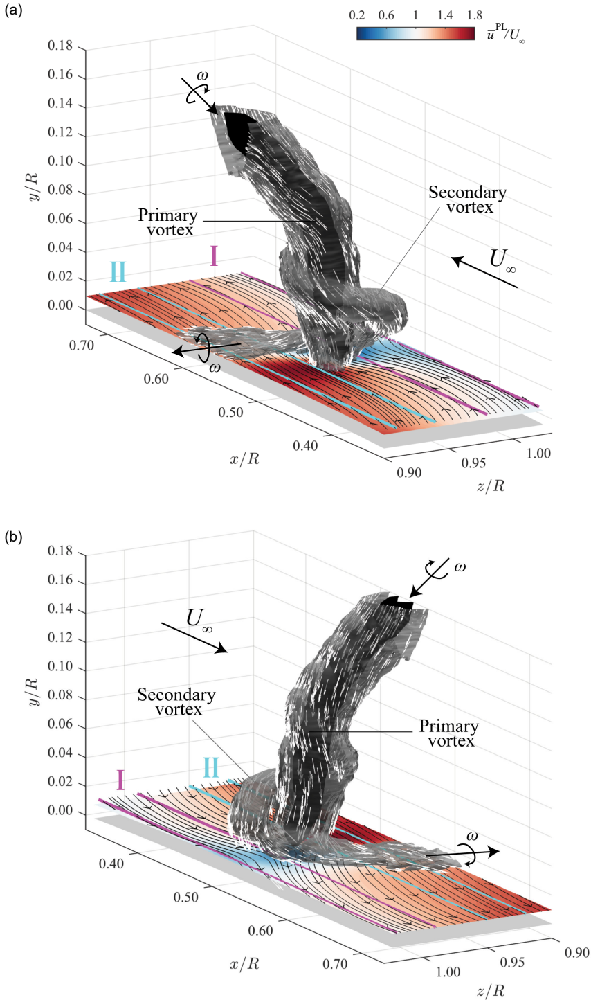
Figure 7. Isosurfaces of vortex core regions for QR^2/U_\infty^2 = 24 (dark grey), 1200 (black) from phase-locked velocity fields at \phi = 80^\circ . White vectors represent local vorticity vectors on the QR^2/U_\infty^2 = 24 isosurface. Surface slices are \bar{u}^{PL}/U_\infty and black lines are streamlines, both at y/\delta_0 = 0.72 . Magenta and cyan lines respectively indicate the outboard (I) and inboard (II) z -locations discussed in § 5.2. (a) Inboard side, downstream view. (b) Outboard side, upstream view.
