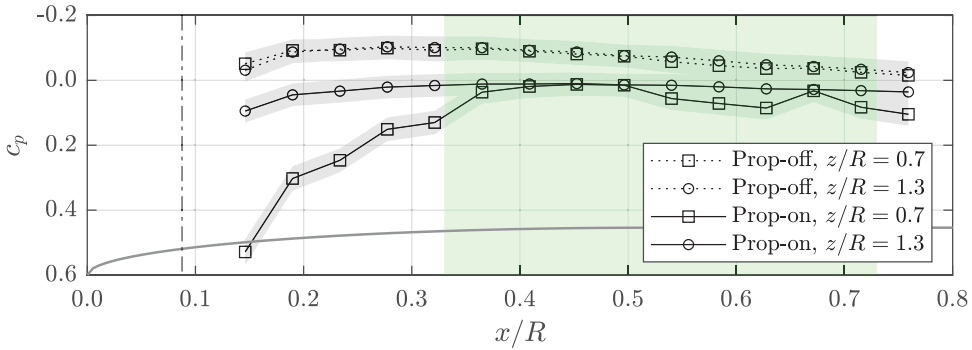
Figure 5. (a) Pressure coefficient distributions for the propeller-on (solid black lines) and off (dotted black lines) cases, with uncertainty represented by the grey shaded regions. Leading-edge geometry is shown as the solid grey line. Shaded green area indicates the PIV measurement domain for the plate-on measurements.
