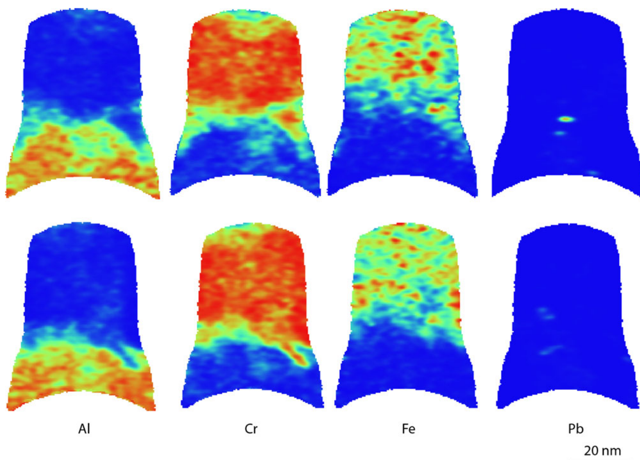
Fig. 7. APT cross-section heatmaps showing the qualitative distribution of Al, Cr, Fe, and Pb in the bottom two layers of the oxide from the material exposed at 600°C. Red indicates high concentration and blue indicates low concentration. The reconstruction was rotated by 90° between upper and lower rows of cross sections. The peak at 27 Da was not used for these maps as there is an overlap between Al, Cr, and Fe.
