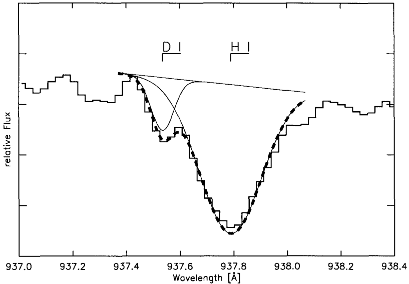
Fig. 2. The ORFEUS II spectrum (histogram mode) with a fit of deuterium and hydrogen Ly- \epsilon (dashed curve) assuming a value of \log(N_D) = 14.7 . Both components and the centers of the absorption lines are indicated. The spectrum has been corrected for the stellar contribution.
