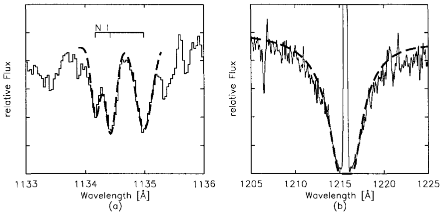
Fig. 1. (a) The NI-triplet at \lambda \approx 1134.5\text{ \AA} in the ORFEUS II spectrum and a fit of the three components is shown (dashed curve). (b) The Ly- \alpha line of hydrogen in the ORFEUS II spectrum of BD +28° 4211 and the theoretical line profile calculated for the value \log(N_H) = 19.8 is presented (dashed curve). In the center of the Ly- \alpha absorption the strong geocoronal emission of Ly- \alpha is visible.
