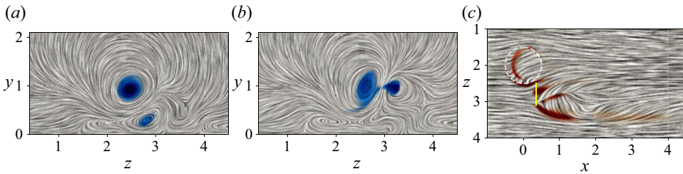
Figure 23. Elliptic flow regions ( \beta < 1 , coloured blue) at x = 2 for cases (a) \Omega_u = 0.75 and (b) \Omega_u = 1.0 . Centrifugally unstable regions ( \gamma < 0 , coloured red) at y = 1.07 for case (c) \Omega_u = 1.31 . The dashed circle in (c) marks the location of the cylinder. Yellow line in (c) for comparison with figure 22(h).
