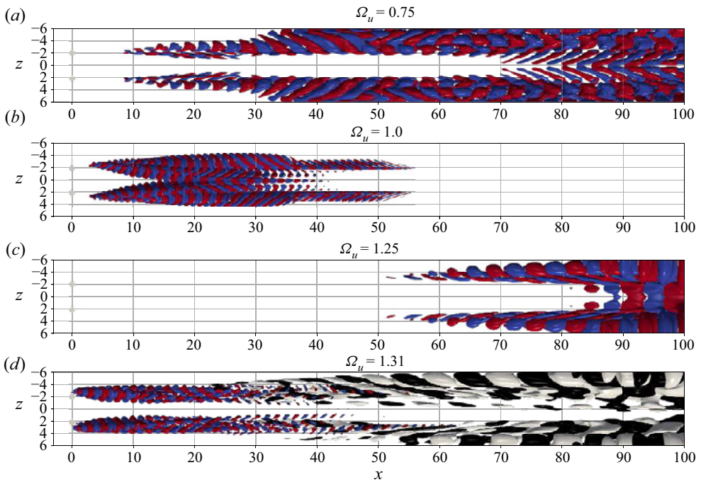
Figure 19. Real part of dominant DMD modes. Frequencies for each mode: (a) \omega_r = 0.92 , (b) \omega_r = 2.2 , (c) \omega_r = 0.66 , (d) primary mode \omega_1 = 1.8 with isosurface in red/blue and second mode \omega_2 = 0.46 with isosurface in white/black. Isosurfaces depict \hat{u} = \pm 10\% (in colour red/blue or white/black) of maximum amplitude of mode.
