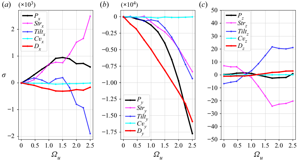
Figure 6. Volume integral of vorticity budget terms in the (a) x-direction, (b) y-direction and (c) z-direction, non-dimensionalised by the corresponding dissipation D_i of case \Omega_u = 0 . Here, P , production; Str , stretching; Tilt , tilting; Cv , convection; D , dissipation terms of vorticity budgets.
