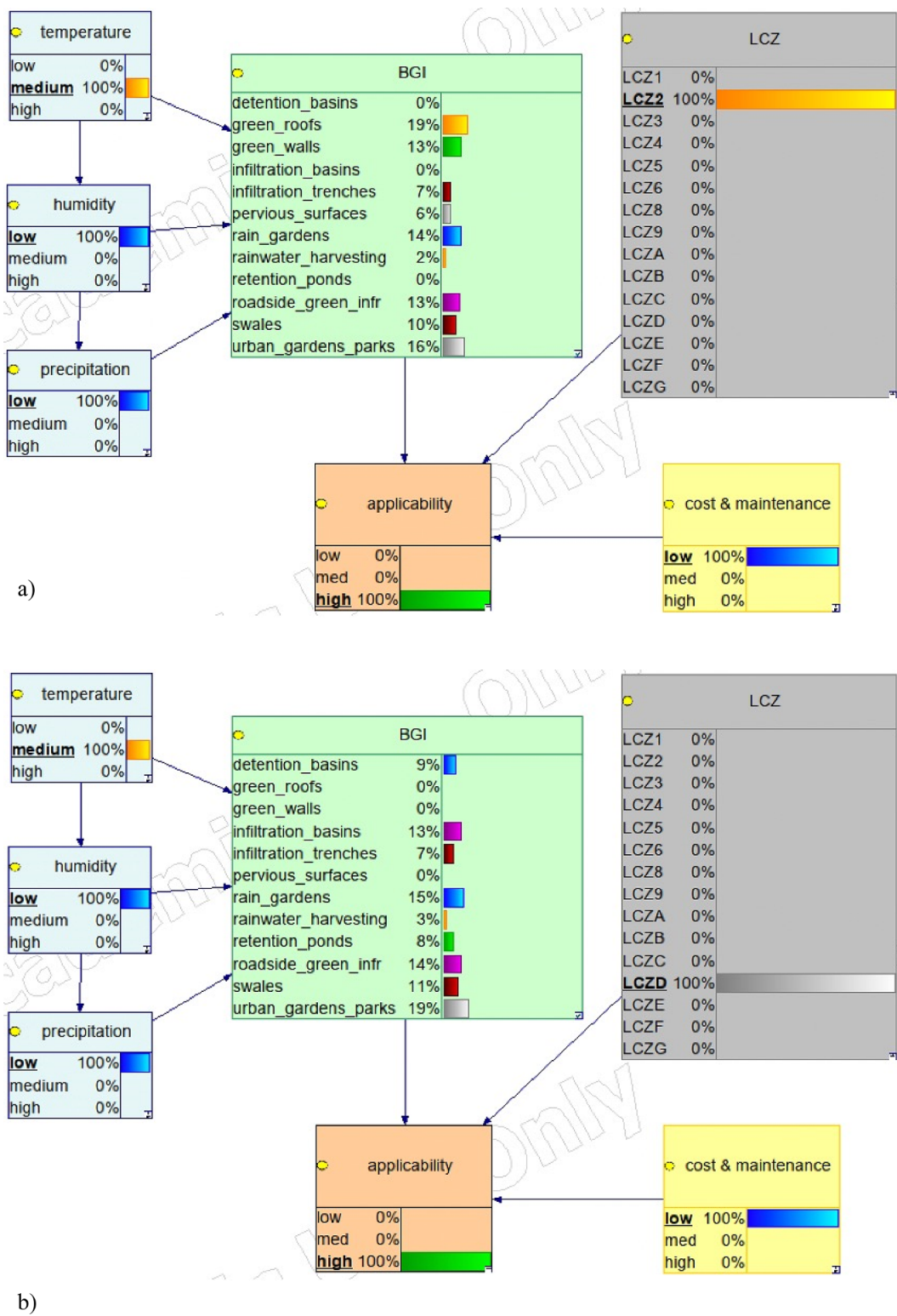
Figure 3. Blue–green infrastructure applicability Bayesian belief network (BGIA-BBN) model a) scenario 1, b) scenario 2.
