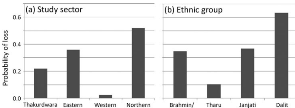
FIG. 2 Probability of livestock loss to leopards by (a) study sector and (b) ethnic group.
