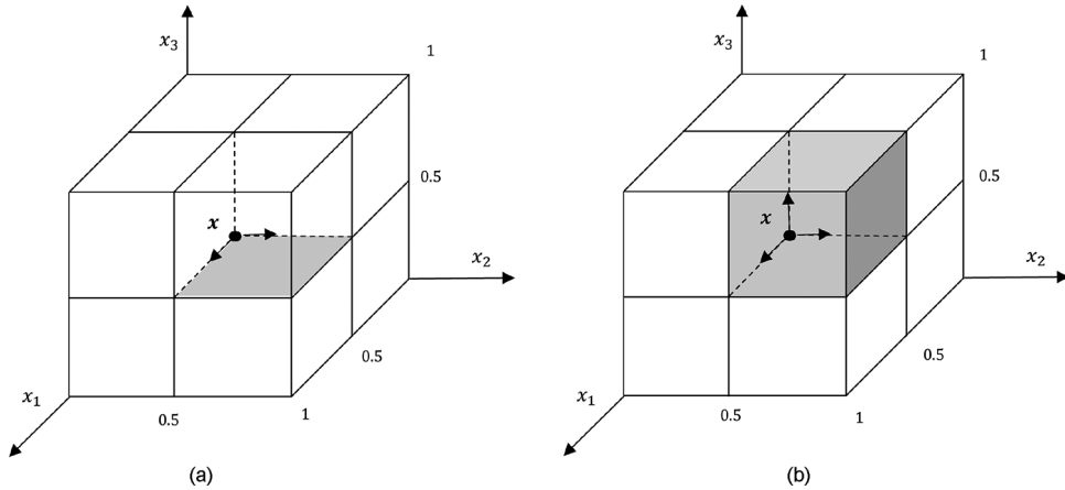
Figure 4. Extension of optimal actions at degradation level \mathbf{x} to higher degradation levels. (a) \mathbf{a}^*(\mathbf{x}, \ell) = (1, 1, 0) in shaded region. (b) \mathbf{a}^*(\mathbf{x}, \ell) = (1, 1, 1) in shaded region.
