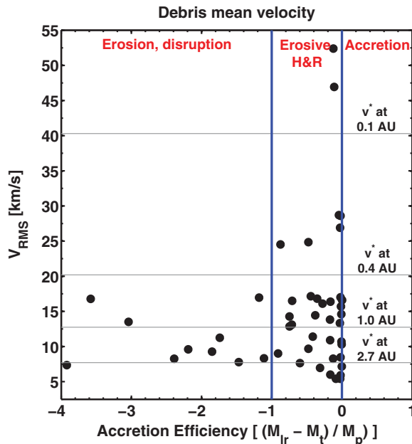
Figure 3. RMS velocity distribution (rock-iron debris, representing mantle and core material), for each set of impact conditions, by collision regime (accretion efficiency parameter). Threshold values (horizontal lines) represent the critical velocity to escape a feeding zone centered at the designated heliocentric distance.
