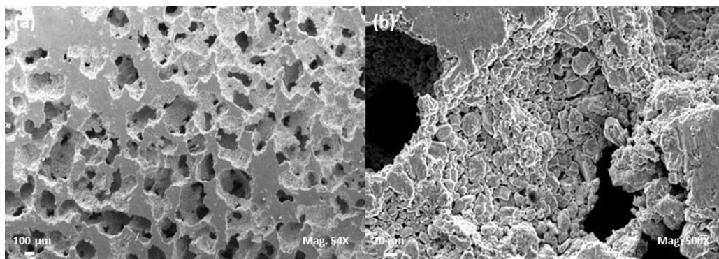
Figure 4. SEM images of foams formed (a) 4 h and (b) 12 h.
