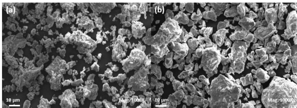
Figure 2. SEM images of Ti-2Nb-4Ta-8Zr powder milled (a) 4h and (b) 12h.
