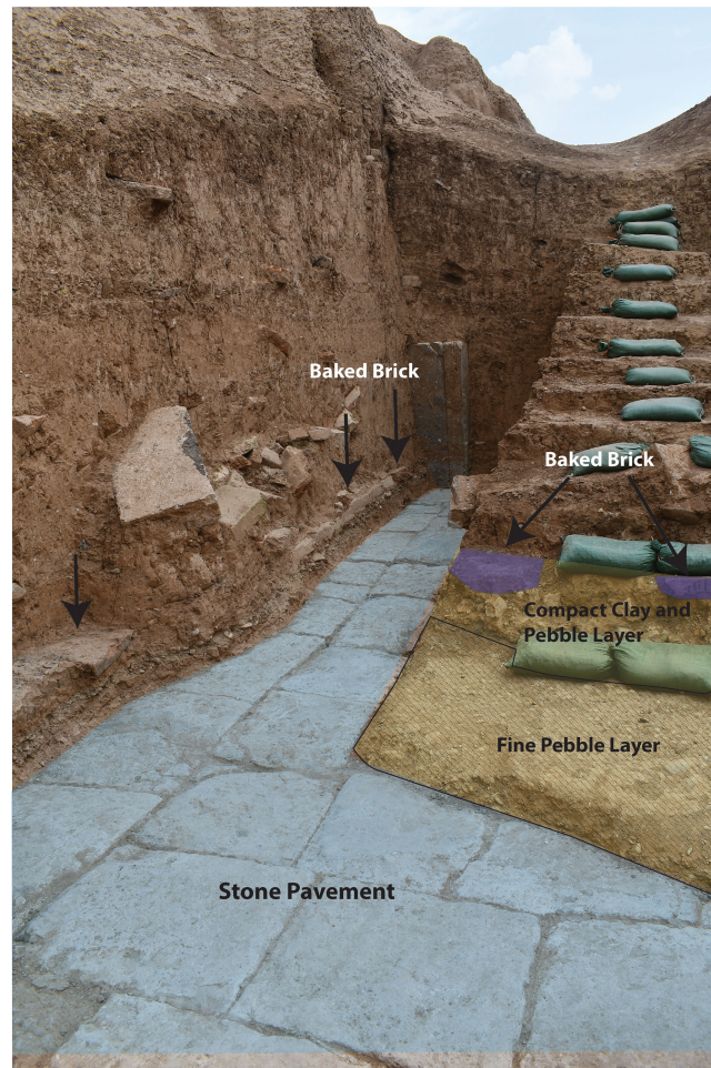
Fig. 10. Details of pavement sequence in operations 1-2
