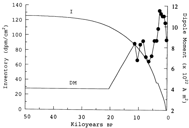
Fig. 2. The standard DM model and the resulting global 14 C inventory, calculated by integrating back in time, so the value at 50 ka BP is actually the present inventory
