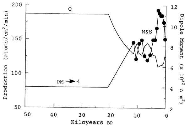
Fig. 1. The standard DM model and corresponding 14 C production function. M&S = McElhinny & Senanyake (1982)
