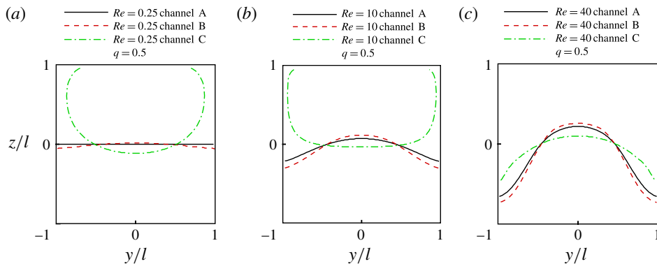
FIGURE 5. (Colour online) Background flow separation lines calculated in cross-section S_c for different side branch geometries at different Reynolds numbers with q = 0.5 . The cross-section S_c is 2l from the entrance, where the flow is already fully developed, and the side branch is going upwards. In the cross-section, the fluid elements above the separation line enter the side branch and those below remain in the main channel. (a) Re = 0.25 ; (b) Re = 10 ; (c) Re = 40 .
