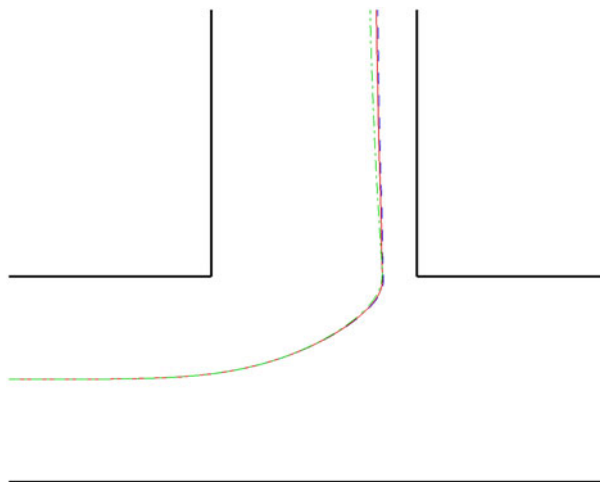
FIGURE 3. (Colour online) Trajectories of a capsule flowing in channel C for a/l = 0.3 , Re = 1 , Ca = 0.005 , q = 0.44 . Different grid resolutions are used: \Delta x = 0.063R (dash-dotted line, green online), \Delta x = 0.04R (solid line, red online), \Delta x = 0.031R (dashed line, blue online). The maximum membrane element edge length is \Delta L_c \sim 0.023l in all cases.
