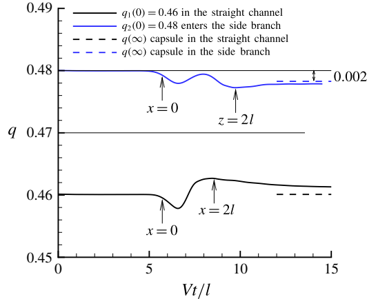
FIGURE 19. (Colour online) Time evolution of the branch flow ratio q in channel C when using constant pressure boundary conditions for a/l=0.3 , Re=20 , Ca=0.1 , q_c=0.47 . The positions of the capsule mass centre in the respective branches are shown by the arrows.
