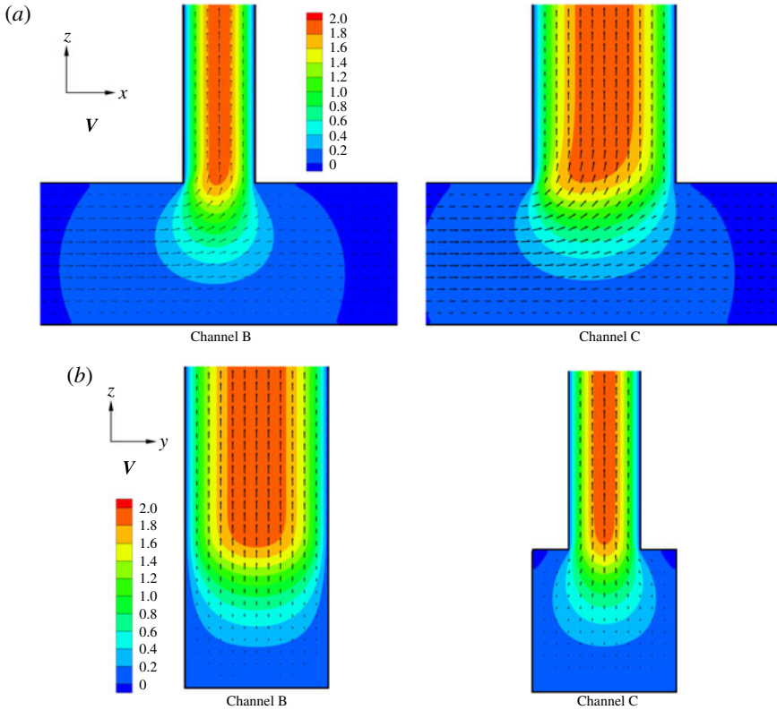
FIGURE 6. (Colour online) Unperturbed velocity field (non-dimensionalised by V ) in the vicinity of the bifurcation for channels B and C. The contours represent the fluid velocity in the z -direction. Re = 0.25 and q = 0.5 . (a) y = 0 -plane; (b) x = 0 -plane.
