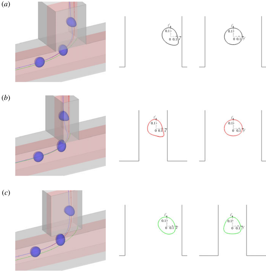
FIGURE 10. (Colour online) Effect of the side branch geometry and confinement on the capsule motion and deformation in channels A, B and C for Re = 20 , Ca = 0.1 , q = 0.7 . The cross-sections of the deformed capsules are shown in two orthogonal planes, using Cartesian coordinate systems centred on the capsule mass centre, with directions x' , y' , z' parallel to the respective directions x , y , z of figure 2. The solid straight lines represent the walls of the side branch.
