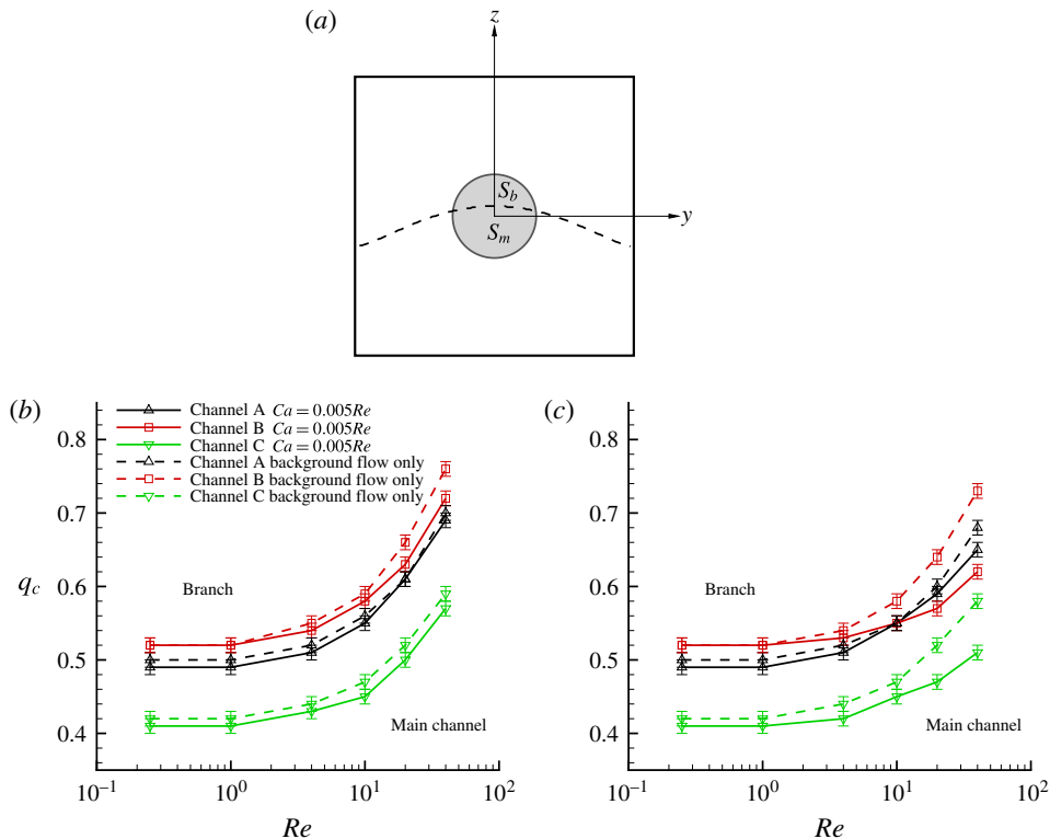
FIGURE 11. (Colour online) (a) Illustration of the definition of the momentum ratio. The dashed line is a fluid separation line (for q = 0.5 , Re = 10 in channel A), which divides the cross-sectional area of the capsule (shaded circle) into two regions, S_b and S_m , the fluid elements of which finally enter the side branch and the downstream main channel, respectively. (b) Phase diagram: critical branch flow ratio as a function of the channel Reynolds number for a capsule with a/l = 0.2 flowing in branched channels with different geometries. Solid lines, full fluid–structure simulations with a capsule (see figure 8); dashed lines, q_{cm} from the background flow only. (c) The same as (b), with a/l = 0.3 .
