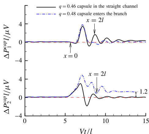
FIGURE 13. (Colour online) Time evolution of the capsule additional pressure drop in channel C under constant flow rate conditions ( a/l = 0.3 , Re = 20 , Ca = 0.1 , q_c = 0.47 ). The positions of the capsule mass centre in the respective branches are shown by the arrows.
