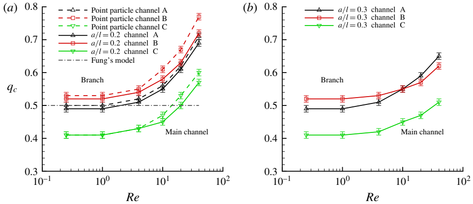
FIGURE 8. (Colour online) Phase diagram: critical branch flow ratio as a function of the channel Reynolds number for capsules with different sizes and membrane shear elasticity ( Ca = 0.005Re ) flowing in branched channels with different geometries. For q > q_c , the capsule flows into the side branch. (a) Comparison of the results for a/l = 0.2 versus a point particle ( a/l = 0 ); (b) a/l = 0.3 .
