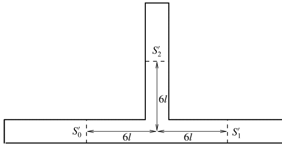
FIGURE 17. Definition of the cross-sections where the pressure is evaluated to determine the pressure drop in the bifurcation.
