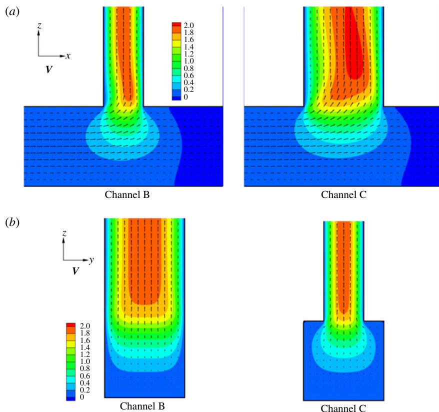
FIGURE 7. (Colour online) The same legend as in figure 6 but for Re = 20 and q = 0.5 .
