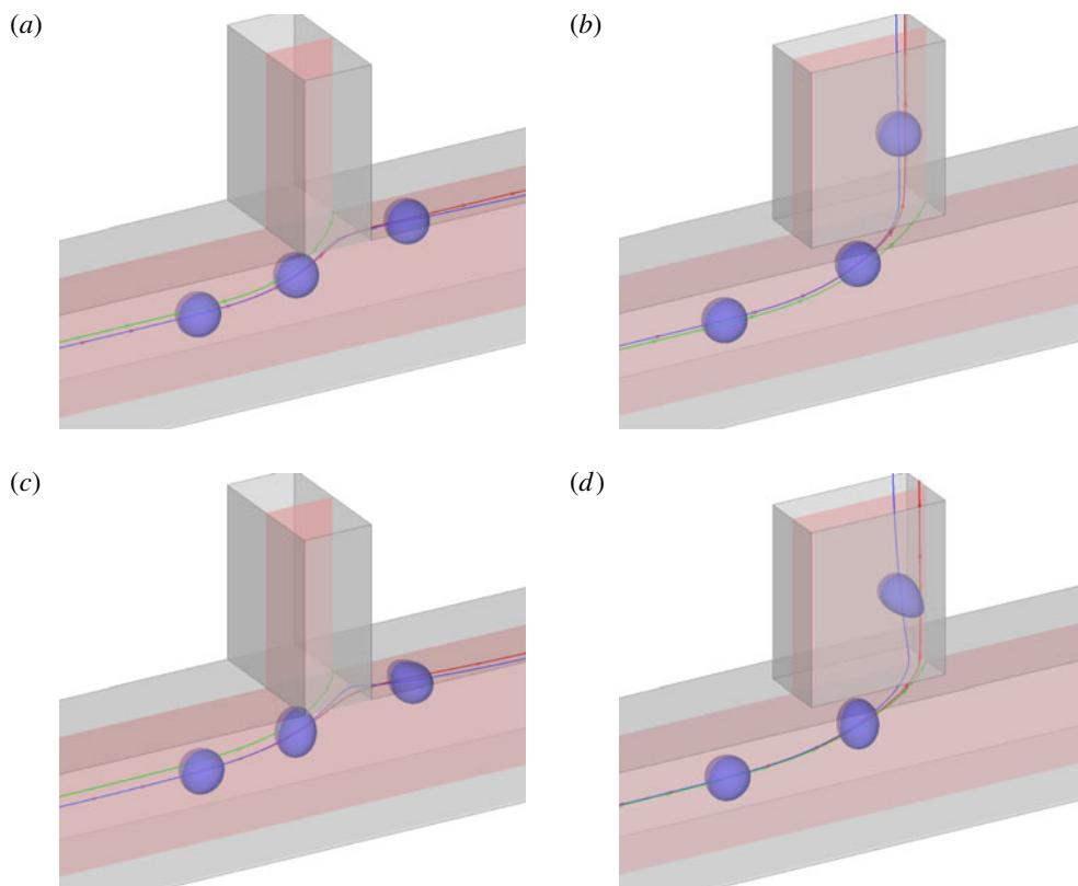
FIGURE 9. (Colour online) Effect of narrowing the side branch on the capsule trajectory in the symmetric xz -plane for a/l = 0.3 . The thick solid line (blue online) represents the trajectory of the capsule centre. The dark line with arrows (red online) represents the unperturbed streamline starting from the centre of S_c in the absence of a capsule, while the grey line with arrows (green online) represents the separating streamlines that divide the fluid elements entering the side branch from those entering the downstream straight channel. (a,b) Re = 1 , Ca = 0.005 , q = 0.46 ; (c,d) Re = 20 , Ca = 0.1 , q = 0.54 ; (a,c) channel B; (b,d) channel C.
