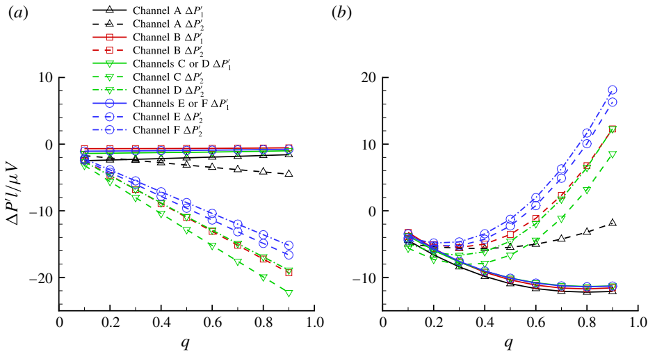
FIGURE 18. (Colour online) The additional pressure drop \Delta P'_1 and \Delta P'_2 (non-dimensionalised by \mu V/l ) due to the bifurcation as a function of the branch flow ratio q in branched channel flows without the capsule. (a) Re = 0.25 ; (b) Re = 20 .
