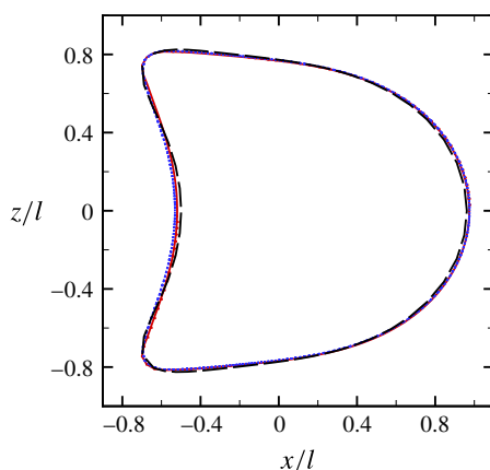
FIGURE 4. (Colour online) Steady profiles of an initially spherical capsule with an SK membrane ( C = 1 ) flowing in a square section channel for a/l = 0.85 , Re = 0.25 , Ca = 0.1 . The bending stiffness of the membrane is, in this case, set to zero to be consistent with Hu et al. (2013). Dotted line (blue online), profile C_1 , obtained with 32 768 flat triangular elements; solid line (red online), profile C_2 obtained with 8192 elements; dashed line (black online), profile obtained by Hu et al. (2013) for Re = 0 , using a boundary element method.
