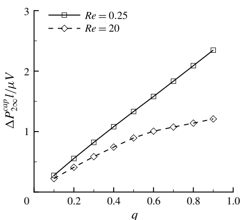
FIGURE 14. Additional capsule pressure drop in a rectangular side branch (section 2l \times l ) as a function of the flow split ratio for a/l = 0.3 , Ca = 0.005Re . Note that Re is defined in the parent channel.
