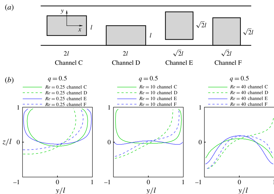
FIGURE 15. (Colour online) (a) Top view of the side branch geometries for channels C, D, E and F. Channels C and E are centre-connected to the main channel. (b) Fluid separation lines for channels C, D, E and F. From left to right: Re = 0.25 ; Re = 10 ; Re = 40 .
