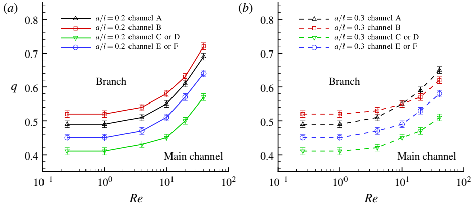
FIGURE 16. (Colour online) Phase diagram: critical branch flow ratio as a function of the channel Reynolds number for capsules in branched channels A, B, C and E. The values of q_c in channels D and F are very close to those in channels C and E, respectively, and are therefore not shown. Ca = 0.005Re . (a) a/l = 0.2 ; (b) a/l = 0.3 .
