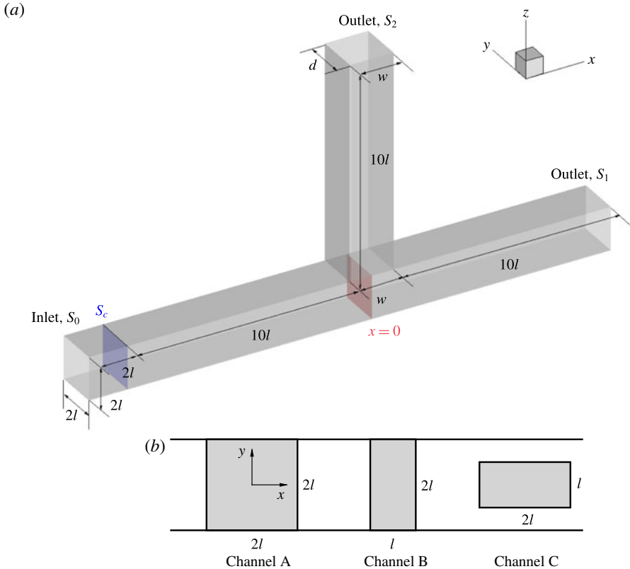
FIGURE 2. (Colour online) (a) Three-dimensional geometry of a branched channel. The width and depth of the side branch are w and d , respectively. (b) Top view of the side branches for channel A ( w = d = 2l ), channel B ( w = l, d = 2l ) and channel C ( w = 2l, d = l ). All side branches are centre-connected to the main channel.
