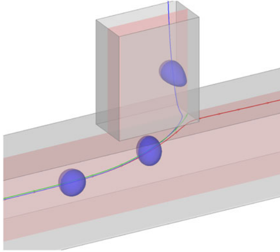
FIGURE 12. (Colour online) Capsule crossing the background flow separation streamline in channel C for a/l=0.3 , Re=20 , Ca=0.1 , q=0.5 .
