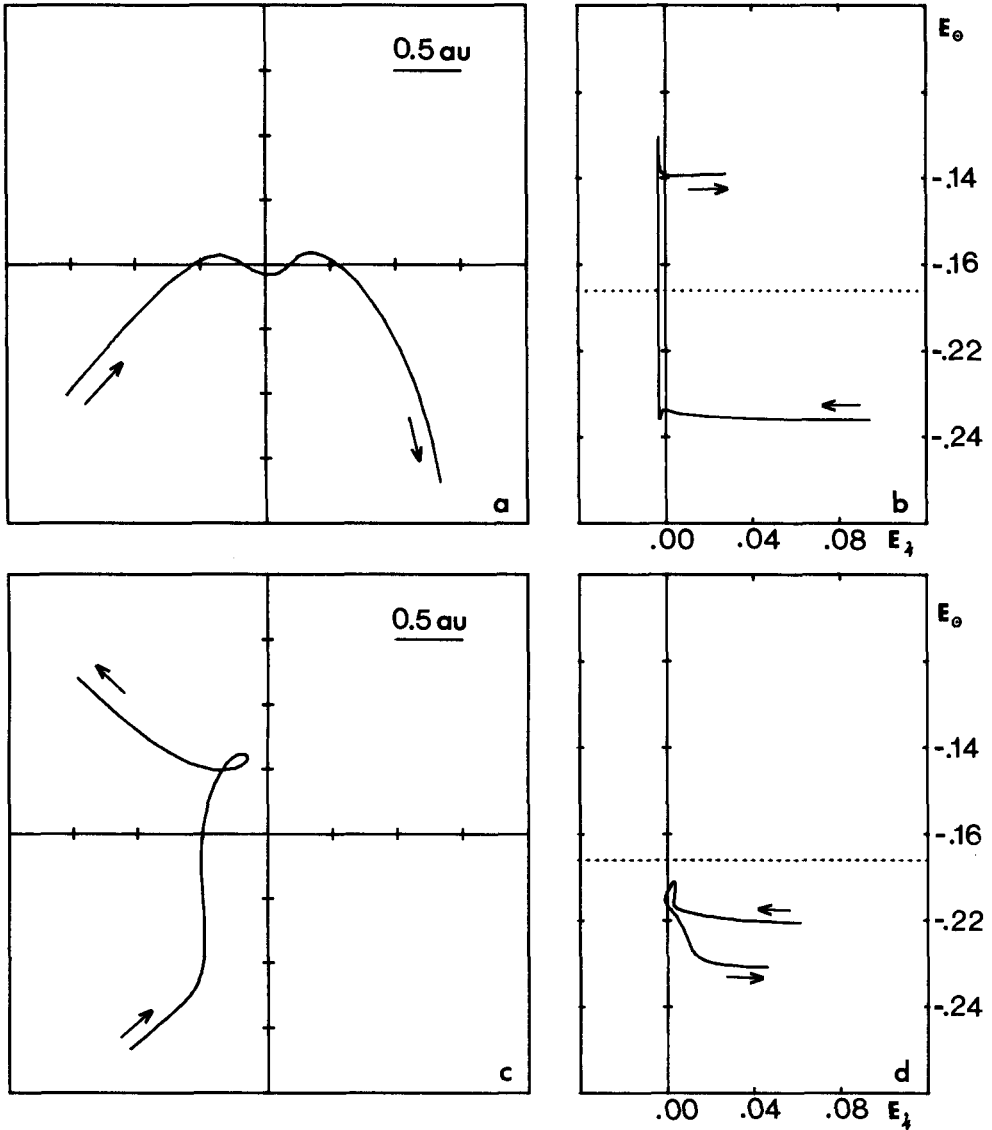
Figure 5. Left: Jovicentric paths in a rotating frame (Sun on the negative x-axis) of P/Oterma (a) during the 1960-1967 encounter and of P/Gunn (c) during the 1870-1884 encounter; tic marks: 0.5 AU. Right: For the same encounters (b: P/Oterma; d: P/Gunn) the heliocentric orbital energy E_{\odot} = -1/a versus the jovicentric one E_J = -m/(Ma') are given, where m is the mass of Jupiter, M that of the Sun, and a' is the jovicentric semi-major axis.
