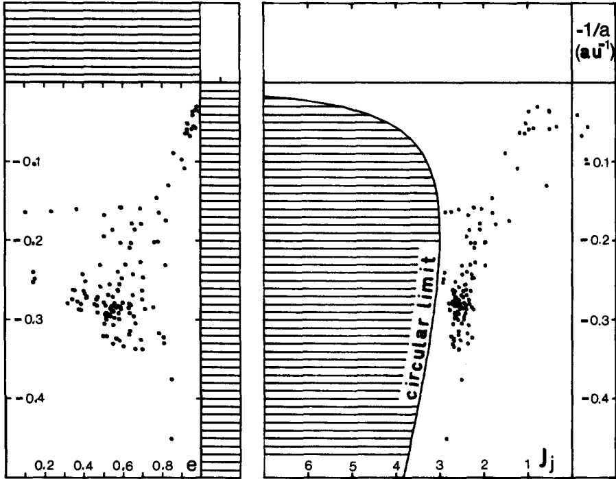
Figure 1. Left: The orbital energy ( -1/a ) of all periodic comets discovered until the end of 1983 is plotted versus their orbital eccentricity e . Right: The same quantity is plotted versus the Tisserand invariant with respect to Jupiter J_j . Forbidden regions are shaded in both plots.
