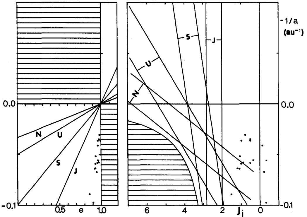
Figure 2. The same as Figure 1, the ordinate being restricted to the outer part of the solar system. The slant lines in the left plot represent orbits tangent in perihelion to those of the planet whose initial labels the line. The pairs of straight lines in the right plot represent orbits whose Tisserand invariant is equal to 2 (line on the right of each pair) and 2.83 (line on the left) with respect to the four outer planets (labels as before).
