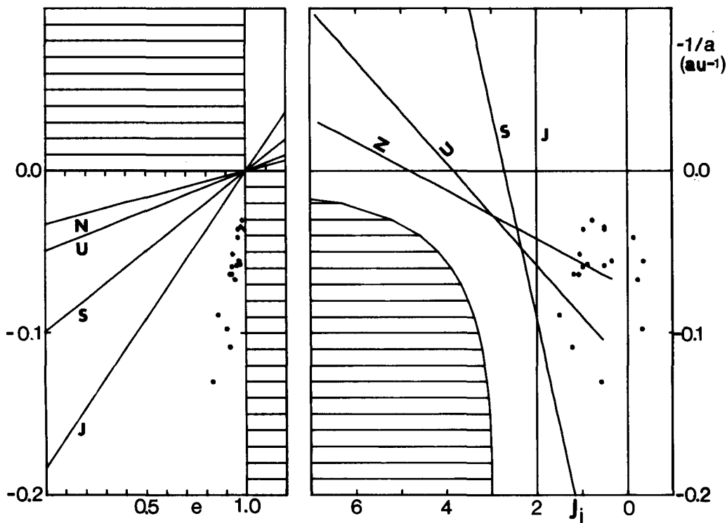
Figure 3. In the same style of Figures 1 and 2, all Halley type comets discovered up to the end of 1983 are indicated. In the right plot only the lines for Tisserand invariant equal to 2 are reported.
