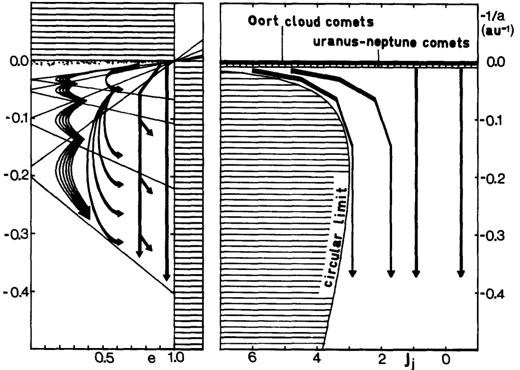
Figure 4. Possible evolutionary paths in the energy-eccentricity and in the energy-Tisserand invariant planes. The leftmost ones in both plots can imply low velocity encounters with all the outer planets in succession; the rightmost ones, leading to Halley type comets, imply mainly encounters with Jupiter; between these two extrema, single-stage captures are possible. The paths are only indicative, and real objects would not follow them strictly. The cometary reservoirs of the outer solar system are indicated by dots in the left plot.
