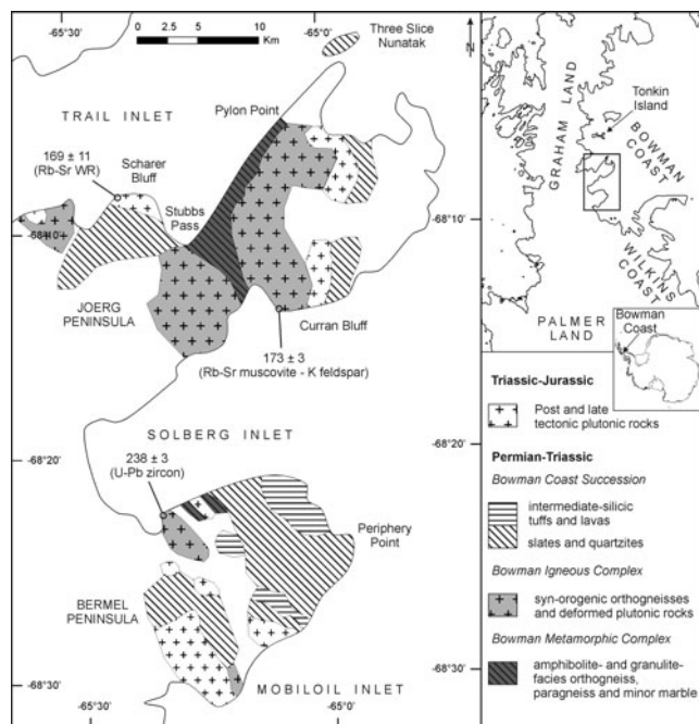
Fig. 1. Geological sketch map for the Bowman Coast showing the location and age of previously dated rocks.
