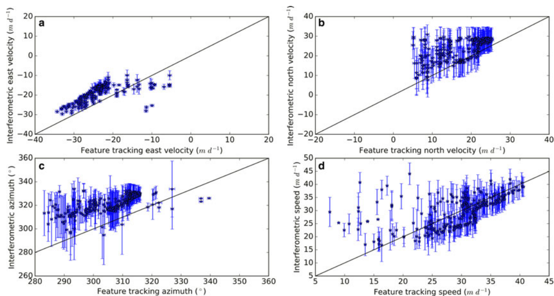
Fig. 4. A pointwise comparison between the overlapping 2-D interferometric and feature-tracking data for components > 5 \text{ m d}^{-1} . The plots compare eastward velocity (a), northward velocity (b), azimuth (c) and velocity magnitude (d). One-to-one relationship lines are shown on every plot. Note that the variability is close to what is described by the Monte Carlo simulation (Figs 6, 7). Error bars show the one SD uncertainties for the interferometric data. The feature-tracking (PIV) uncertainty is assumed to be 0.1 pixels (0.2 \text{m d}^{-1} (0.5 m over a 3-day period, to one significant figure) for each of the velocity components. The feature-tracking uncertainty error bars for the magnitude and azimuth are derived from another Monte Carlo simulation.
