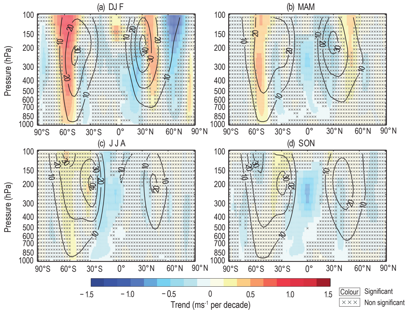
Figure 2.18 | Trends in ERA5 zonal-mean zonal wind speed. Shown are (a) DJF (December–January–February); (b) MAM (March–April–May); (c) JJA (June–July–August); and (d) SON (September–October–November). Climatological zonal winds during the data period are shown in solid contour lines for westerly winds and in dashed lines for easterly. Trends are calculated using OLS regression with significance assessed following AR(1) adjustment after Santer et al. (2008) ('x' marks denote non-significant trends). Further details on data sources and processing are available in the chapter data table (Table 2.SM.1).
