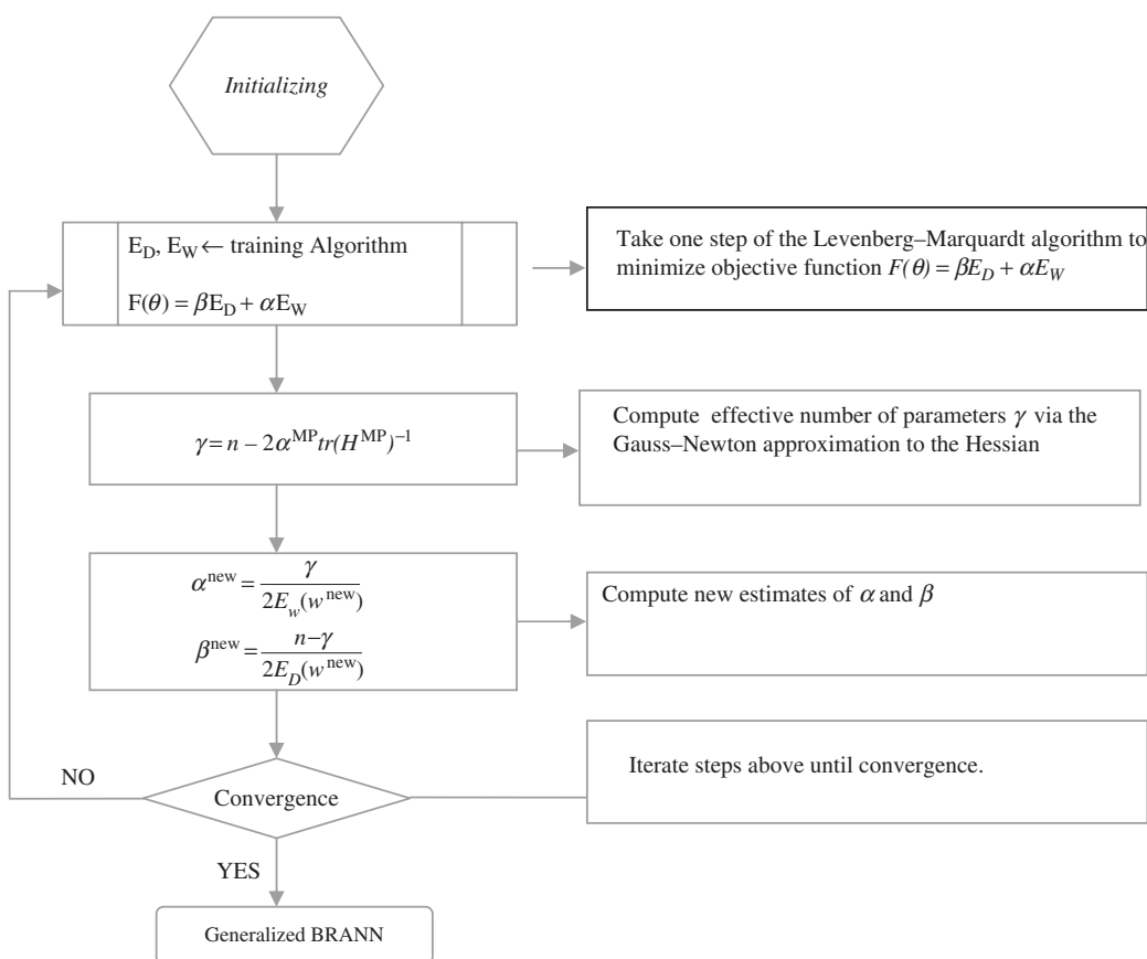
Fig. 2. Flow chart for Bayesian optimization of regularization parameters \alpha and \beta in NNs; MP, maximum a posteriori (adapted from Shaneh & Butler, 2006).
