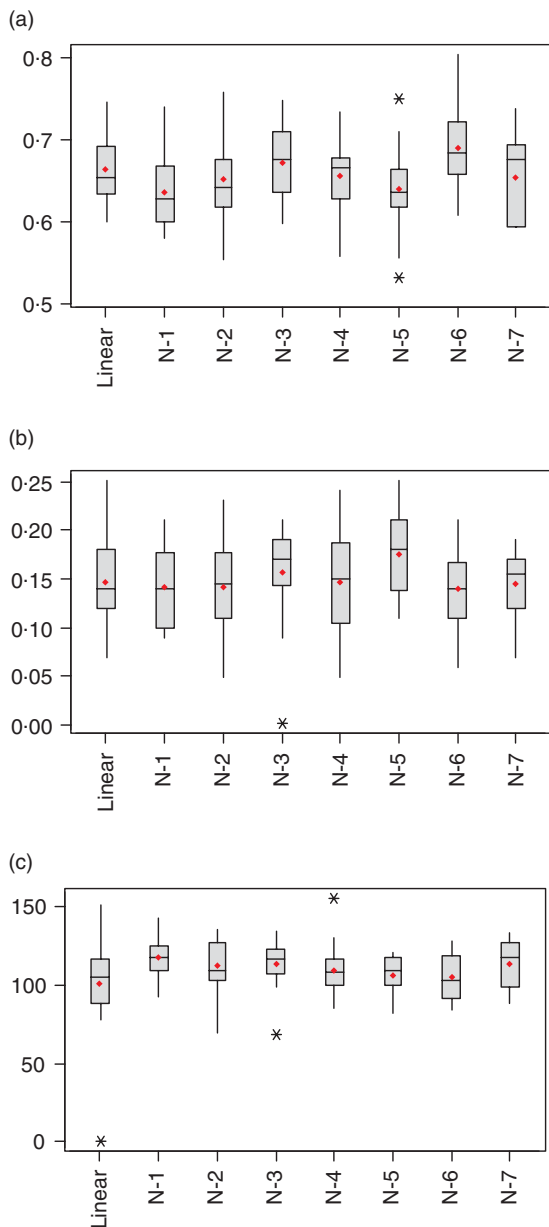
Fig. 3. Box-plots for (a) mean-squared error in the testing set, (b) correlation between predictions and observations in the testing set and (c) effective number of parameters, \gamma , after 20 independent runs (*indicates extreme values).
