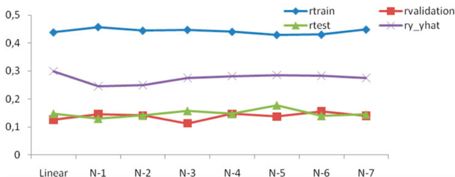
Fig. 4. Correlations between predictions and observations for training ( r_{\text{train}} ), testing ( r_{\text{test}} ), tuning ( r_{\text{validation}} ) and overall ( r_{y-\hat{y}} ) for linear and seven ( N-1-N-7 ) network architectures.
