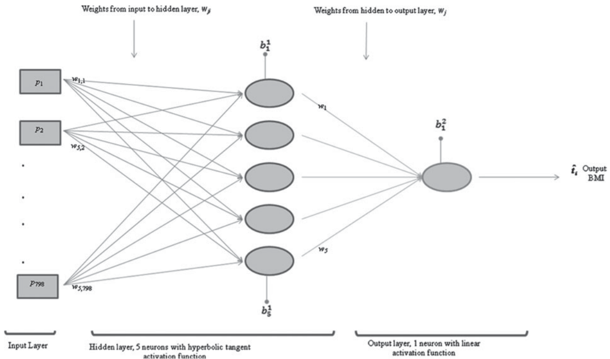
Fig. 1. ANN design used in this study. There were 798 SNP genotypes used as inputs ( p_{ij} ). Each SNP is connected to up to five neurons via coefficients w_{jk} ( j denotes neuron, k denotes SNP). Each hidden and output neuron has a bias parameter b_j^{(l)} , j denotes neuron, l denotes layer).
