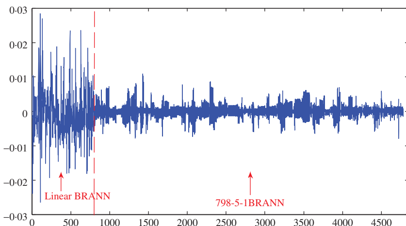
Fig. 5. Distribution of weights ( w_{kj} ) for the linear model and for neural network with five neurons.
