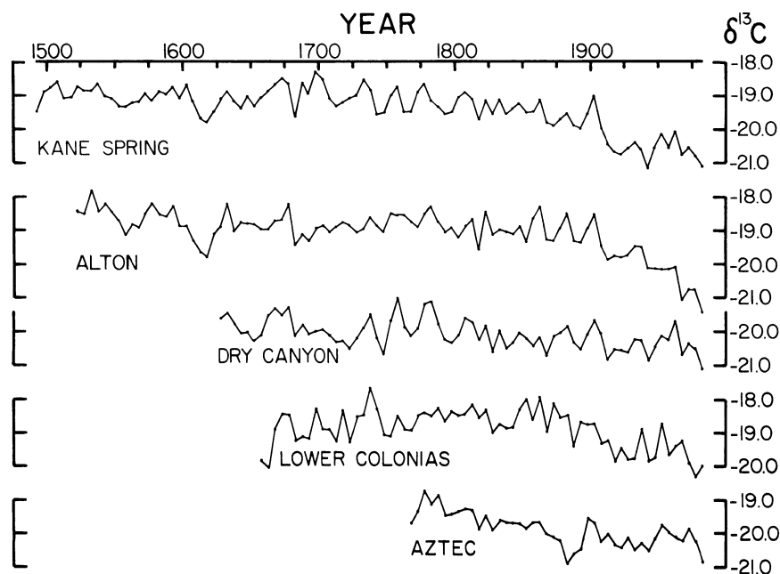
Fig 2. The δ 13 C curves from the 5 sites each derived from analysis of a composite sample produced by pooling 4 cores from each of 4 trees
