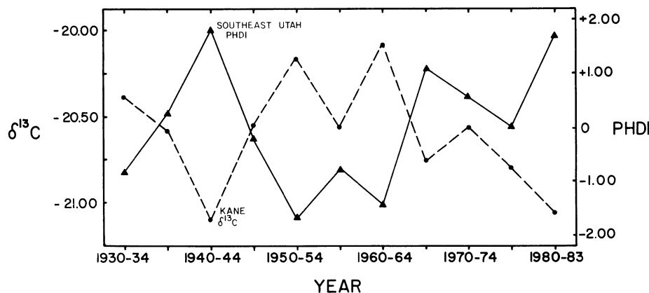
Fig 3. Plot of Kane Spring \delta^{13}\text{C} data (●) and the 5-yr mean Palmer hydrologic drought indices (PHDI) (▲) for the post-1930 period. The first point on the PHDI curve is actually 1931–34 and the last point is 1980–82.
