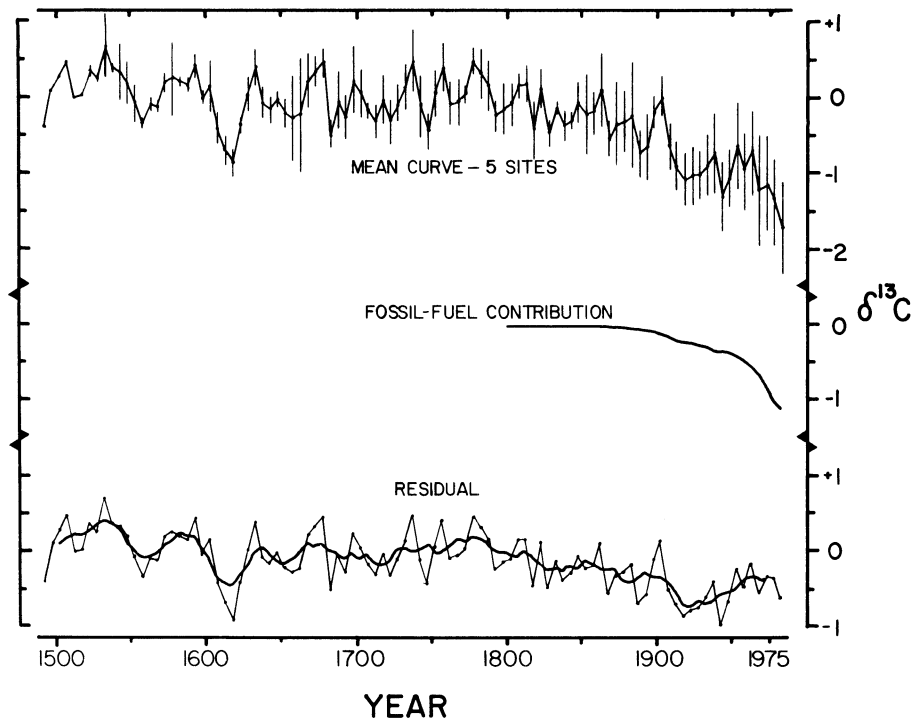
Fig 4. The mean \delta^{13}\text{C} curve from the 5 sites (upper curve), the portion of atmospheric \delta^{13}\text{C} trend attributed to fossil-fuel consumption (middle curve after Peng et al , 1983), and the residual difference representing apparent biospheric activity (lower curves, unsmoothed and smoothed)
