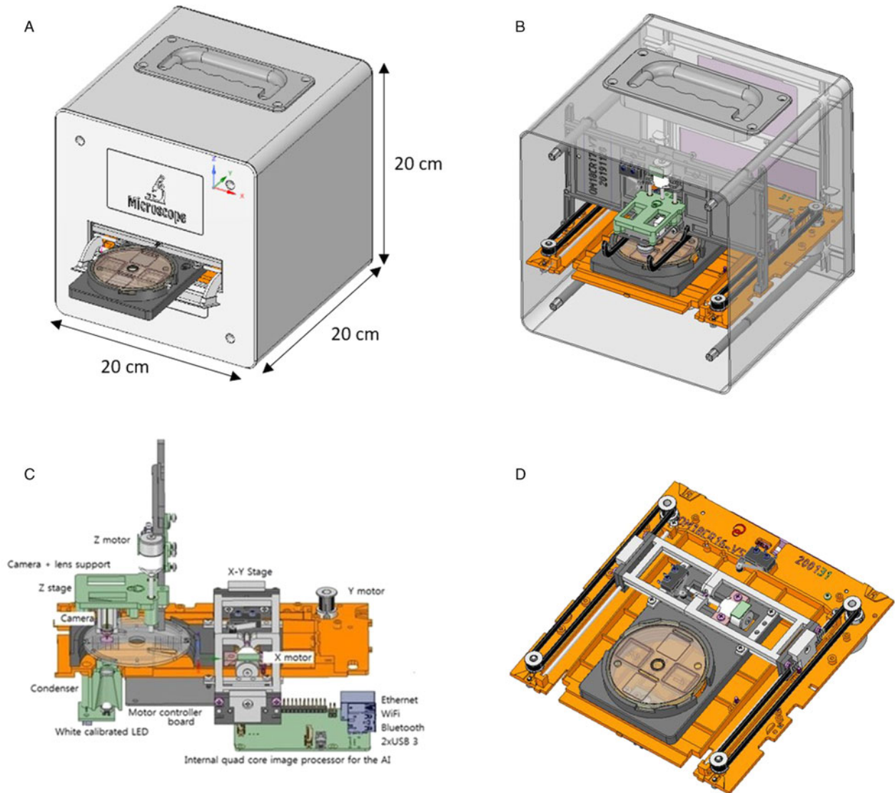
Fig. 2. (A) FreeCAD and Design Spark Mechanical of the KFM (external view); (B) FreeCAD and Design Spark Mechanical of the KFM (internal view); (C) schematic diagram showing mechanical, electronic and optical systems of the KFM and (D) a particular of the handling motor based on the no-standard Cartesian system.
