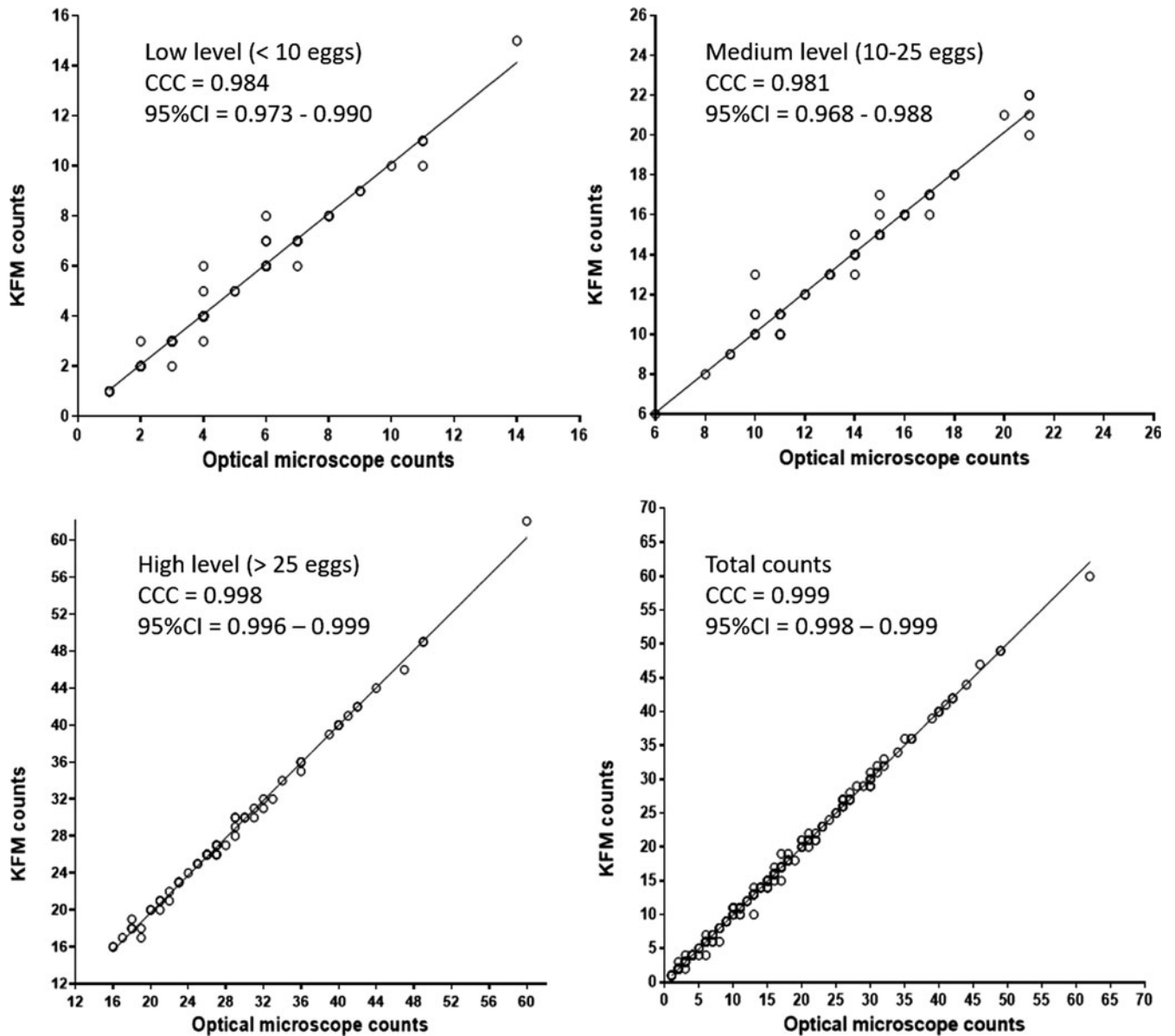
Fig. 6. Correlation between the number of counted eggs based on the examination of Mini-FLOTAC using the OM and KFM for each level of egg counts and total counts.
