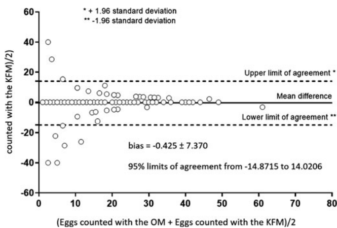
Fig. 7. Bland-Altman plot of number of counted GIN eggs based on the examination of Mini-FLOTAC using OM and KFM.
