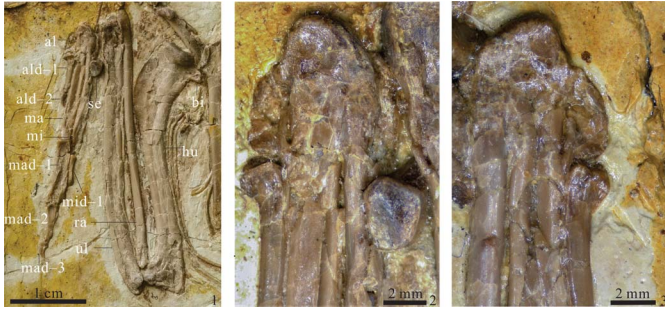
Figure 10. Left forelimb of the holotype (MHGU-3000) of Musivavis amabilis n. gen. n. sp. in ventral view. (1) Photograph; (2) close-up of the proximal ends of the left metacarpals; (3) close-up of the proximal ends of the right metacarpals. Abbreviations: al, alular metacarpal; ald-1–2, alular digit 1–2; bi, bicipital crest; hu, humerus; ma, major metacarpal; mad-1–3, major manual digit 1–3; mi, minor metacarpal; mid-1, minor manual digit 1; ra, radius; ul, ulna; se, semilunate carpal.
