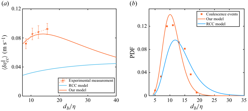
Figure 8. The mean coalescence velocity \langle \delta v_{cc}^{\parallel} \rangle and the size distribution of bubble pairs undergoing coalescence. (a) The mean \langle \delta v_{cc}^{\parallel} \rangle calculated from the coalescence efficiency \mathcal{E}_{cc}^T and the PDF of \delta v_c^{\parallel} . Predictions by our model and the RCC model (Ross 1971; Chesters 1975; Coualaloglou 1975) are shown for comparison. The experiment measured \langle \delta v_{cc}^{\parallel} \rangle is also plotted to validate our model. (b) The size distribution of bubble pairs involved in coalescence events predicted by our model and the RCC model.
