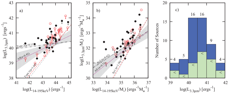
Figure 1. (a) \log(L_{14-195\text{keV}}) versus \log(L_{3.3\mu\text{m}}) and (b) \log(L_{14-195\text{keV}}/M_{\text{BH}}) versus \log(L_{3.3\mu\text{m}}/M_{\text{BH}}) relations. Open red circles are used for Optical type 1 objects and filled black circles for Optical type 2 objects. Arrows are for upper-limits. The best-fit lines from linear regressions with upper limits are also shown. (c) Distribution of \log(L_{3.3\mu\text{m}}) .
