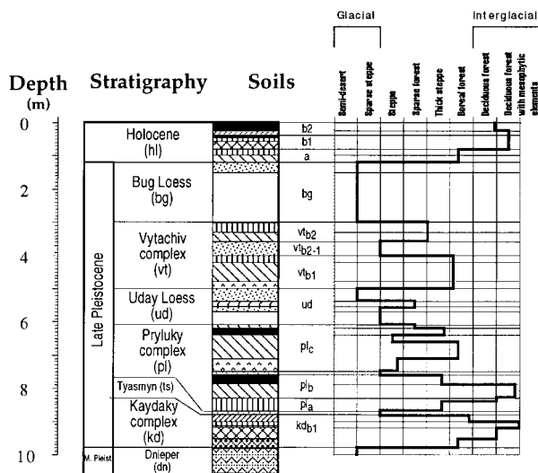
FIG. 4. Stratigraphy, soils, and paleoenvironments of the Vyazivok section. Environmental reconstructions are based on soil and pollen analyses. See Fig. 2 for key to stratigraphic units and soils.
