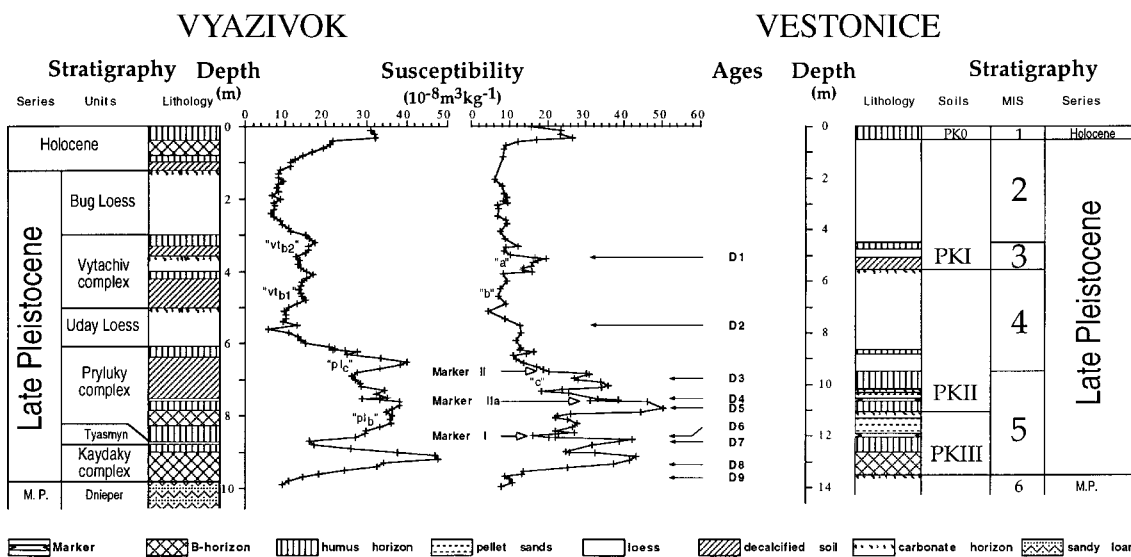
FIG. 5. Correlation of the late Pleistocene Vyazivok sequence, the Vestonice (Czech Republic) loess section, and marine isotope stages. Ages (D1–D9) are given in Table 2. The open arrows indicate the location of the marker horizons identified by Kukla (Kukla and Cilek, 1996).
